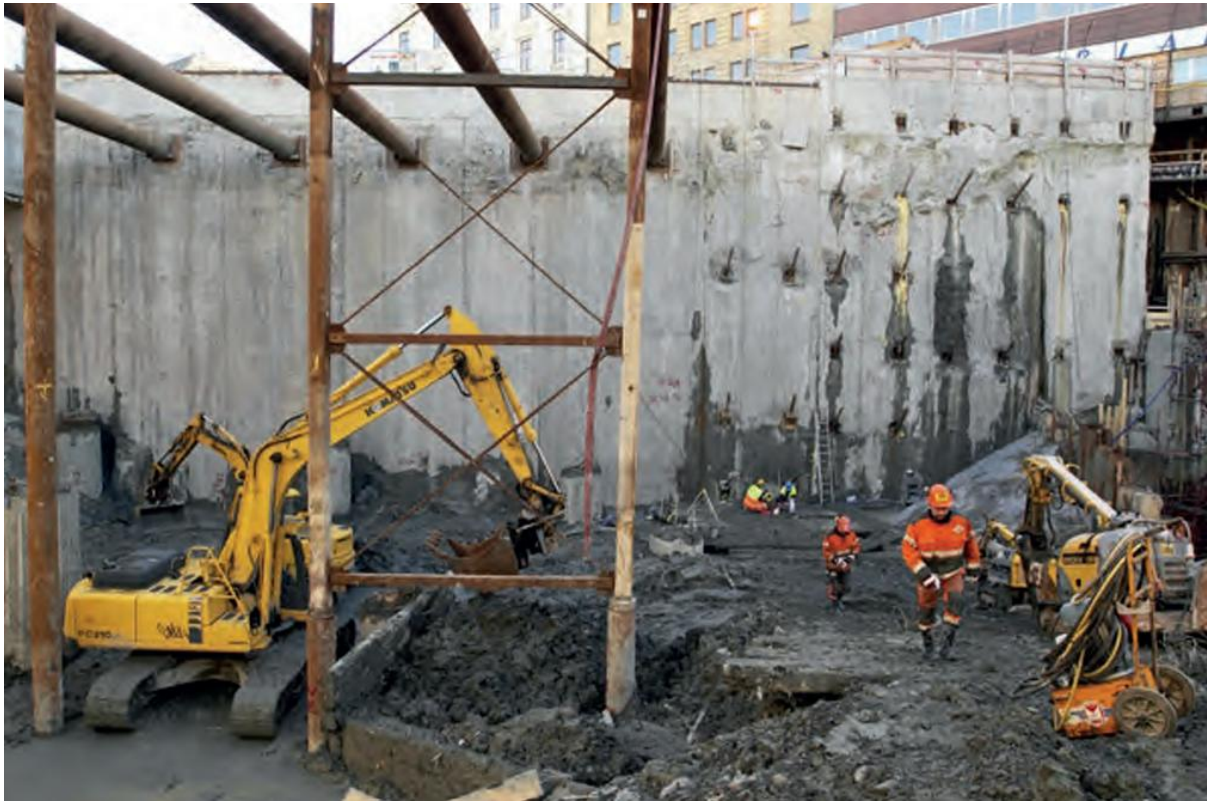
Figure 2.2. Diaphragm walls supported by struts (transverse steel pipes). Source: Trafikverket (2016).
