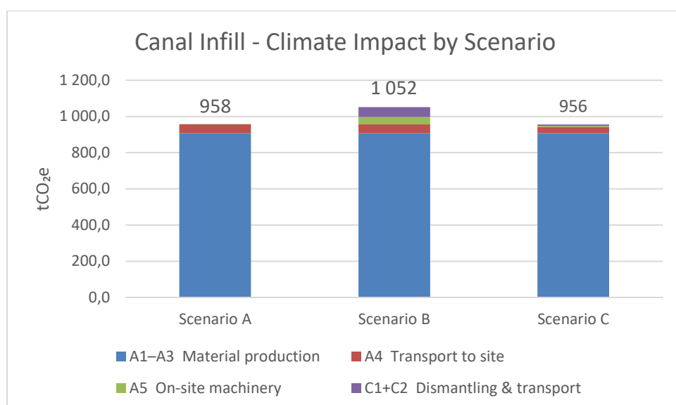
Figure 4.1 The canal infill is dominated by the sheet pile walls, which account for approximately 90% of A1-A3 emissions in all three scenarios. Scenario B is higher than Scenario A due to the addition of A5 machinery and C1+C2 posts absent from the standard calculation. Scenario C returns to a level close to Scenario A, as the confirmed HVO100 fuel for all on-site machinery and dismantling reduces the added emissions substantially.
