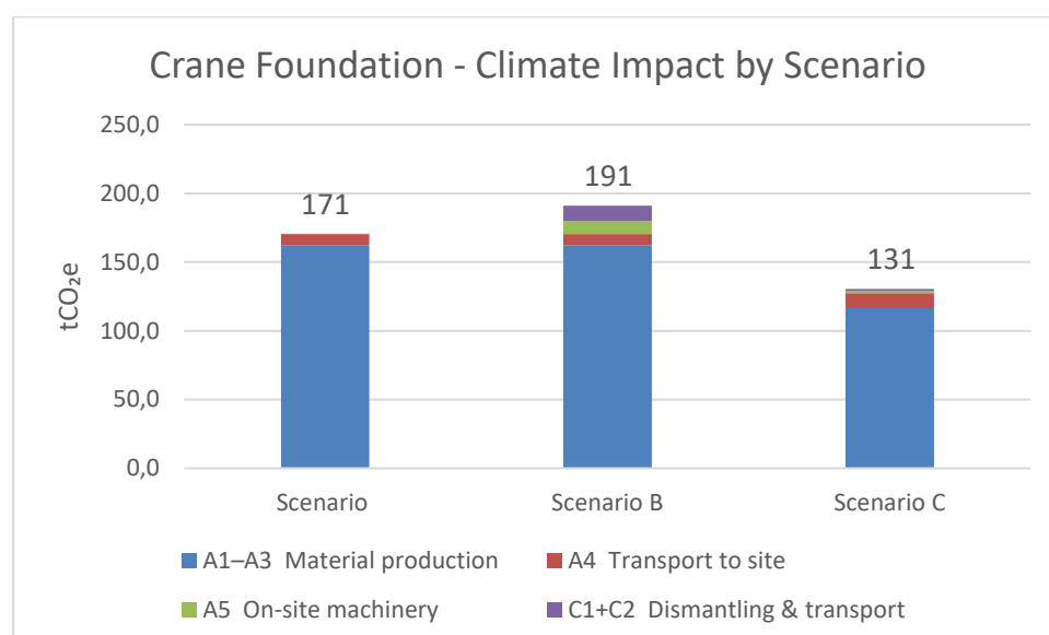
Figure 4.2 The crane foundation results are dominated by A1-A3 material production in all three scenarios, with concrete and reinforcement steel as the primary contributors. The A→B increase reflects the addition of excavation and construction machinery. The significant B→C reduction is driven by the application of project-specific EPDs for both concrete (270 kg CO 2 e/m 3 vs C32/40 generic default value) and reinforcement steel (B GROUP STEEL EPD), which together reduce A1-A3 by approximately 46 tCO 2 e.
