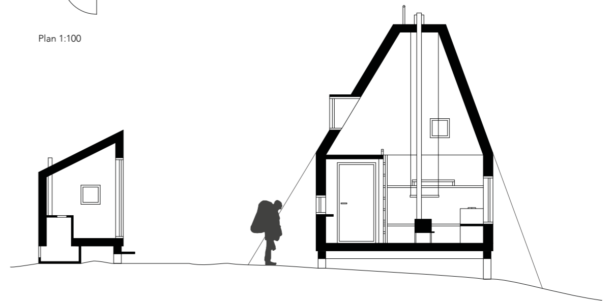
Section 1:100
