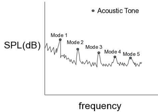
Figure 2.8: Rossiter modes in a spectrum (random data)
