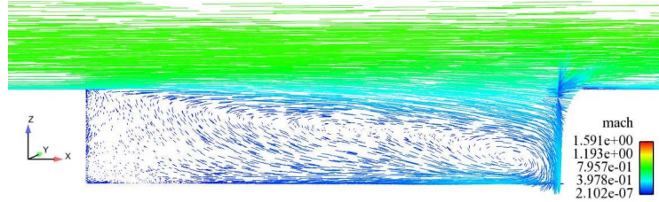
Figure 5.10: Mean velocity vectors colored with mach number on the central section y/W = 0
