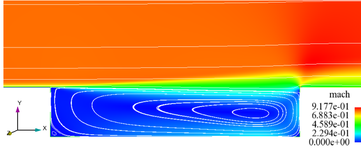
Figure 5.4: Streamlines with mach number contours on the central section y/W = 0 for EARSIM
