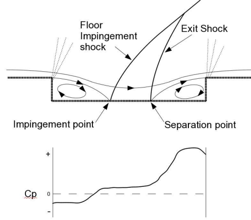
Figure 2.3: Super-sonic closed cavity flow with pressure distribution on cavity floor
