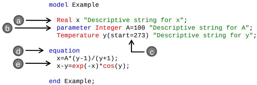
Figure 2.1 Sample Modelica class
