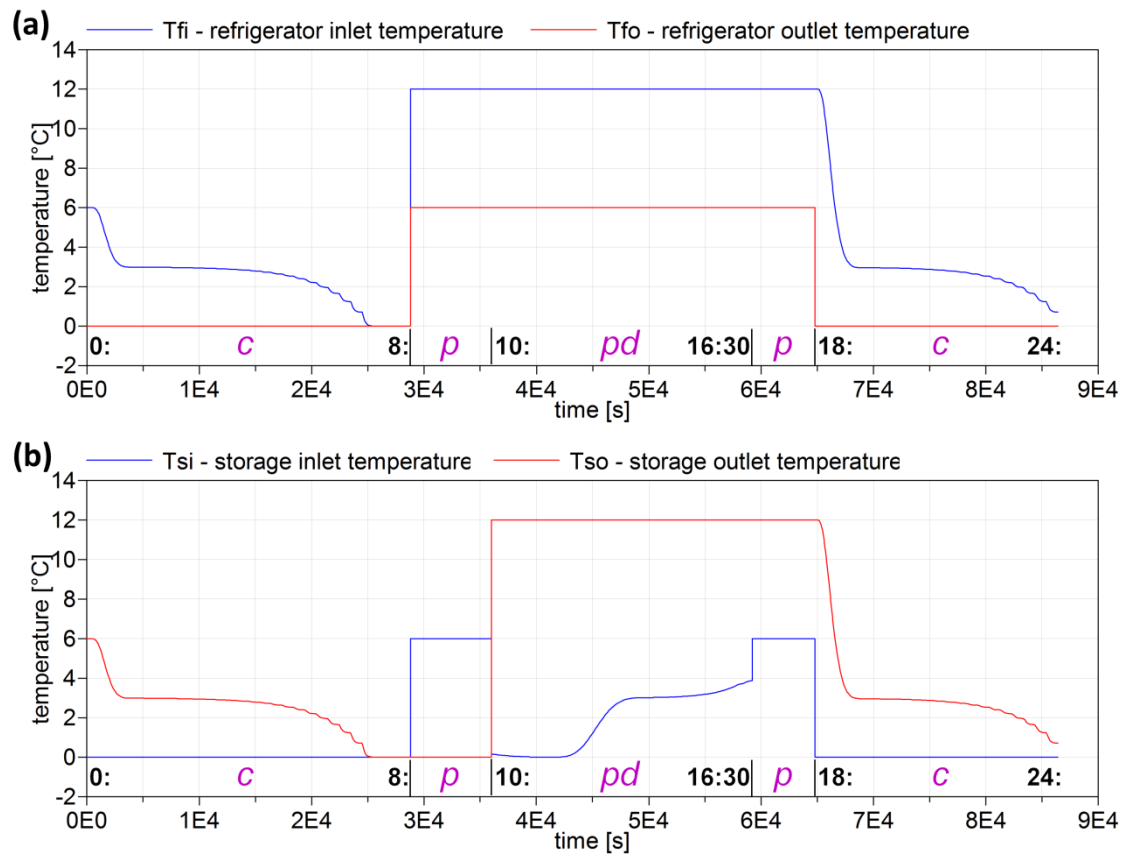
Figure 6.11 Temperatures of (a) the refrigerator and (b) the storage
