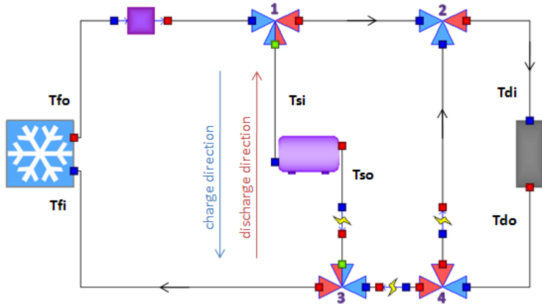
Figure 6.7 Diagram view of the refrigerator and storage network model
