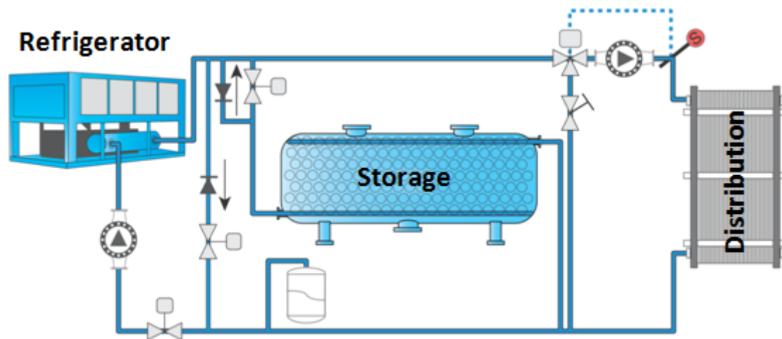
Figure 6.1 Parallel lay-out of a refrigerator and storage network (Cristopia, 2008)
