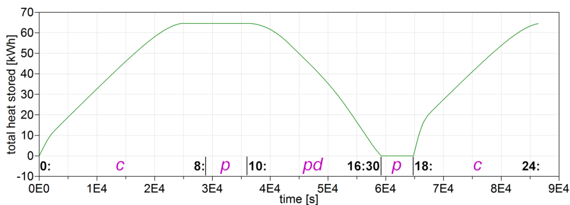
Figure 6.10 Total heat stored in the tank
