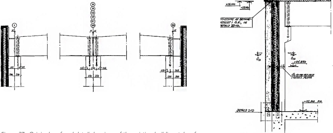
Figure 27. Original roof and detail drawings of the existing building, taken from Mölndal Municipality.
