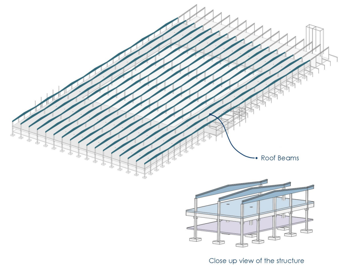
Figure 26. Structural elements of the existing building.
