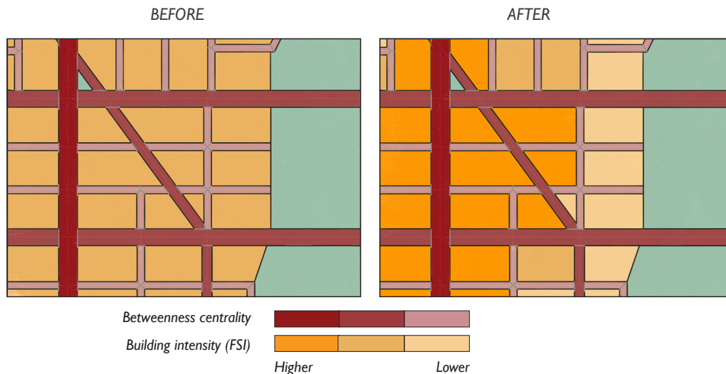
Figure 22: A visual overlay showing the FSI of the built surfaces (occupation surfaces) as well as the Betweenness centrality of the street surfaces, comparing before (left) and after (right) the application of building height and rules.
