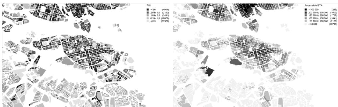
Figure 15: Two maps measuring density using the area measure (left) and the accessible density measure (right). (from Berghauser Pont & Marcus, 2014)
