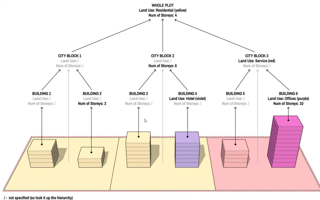
Figure 20: The top-down approach used in the Modelur software, where the properties of Land use and number of stories are inherited from the top level down. (From Modelur, 2024)
