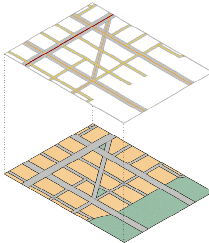
Figure 3: The two constituent layers of the model separated, with the network layer on top and surface layer below.
