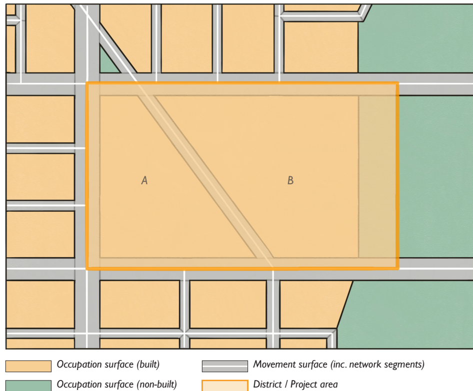
Figure 14: The project area "East" starts out as two separate islands A and B, bounded by streets and a section of park to the east.
