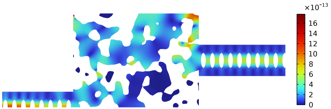
Figure 5.10: This figure shows the magnitude of the displacement of the device in action. As mentioned previously, only half of the device was simulated due to the symmetry. This gives further confirmation that the output waveguide is excited in the correct mode, and that the beamsplitter works as intended.
