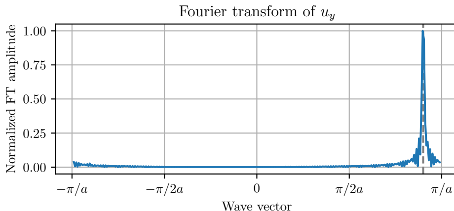
Figure 5.2: Fourier transform of the y-component of the displacement field. It clearly shows one wave traveling forward with a k -vector of 0.9\pi/a , where the dashed gray line is. Since the closest other mode at this frequency is at k_y \approx 0.4\pi/a , where no peak is visible, it is concluded that solely the desired mode is excited.
