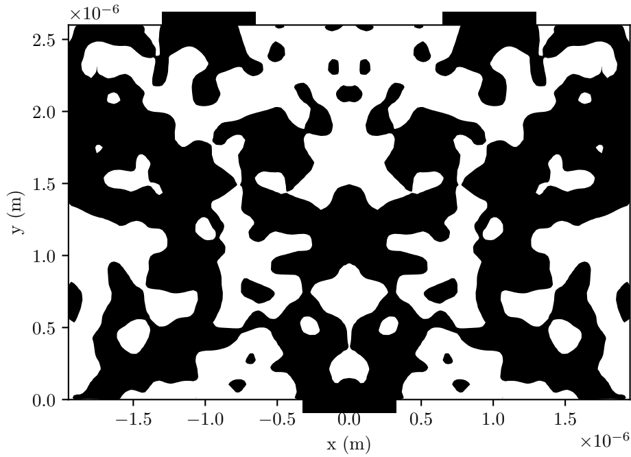
Figure 5.9: This figure shows the final optimized design for the level-set optimization. The device performs a roughly 46/46 split of the incoming power, with the rest of the power being reflected.
