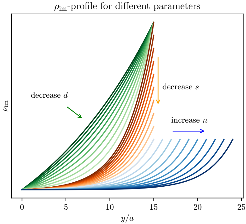
Figure 4.2: This figure shows the effect of changing the different parameters in equation (4.6). The green curves show changing d while keeping the other parameters fixed, and the orange and blue show s and n respectively. Darker colour means higher value, and the last green curve coincides with the first orange, and the last orange with the first blue.
