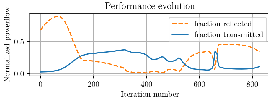
Figure 5.4: Non-converging optimization example. The blue curve shows the transmitted power in one of the output arms as a function of iteration, while the yellow shows the power reflected back out through the input. The cases where two times the blue plus the yellow isn't 1.0 is explained by power exiting through a different mode.
