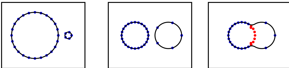
Figure 4.4: Possible evolution of boundary. In the leftmost figure, the boundary is defined by pretty much evenly spaced points. In the center figure the boundaries have moved and the spacing is no longer even, and the right circle is very poorly resolved. The rightmost figure shows the boundary after the two circles moved closer together. Now there are multiple points that need to be removed, marked in red, and the connectivity of the points that remain must be changed such that the two boundaries are merged.
