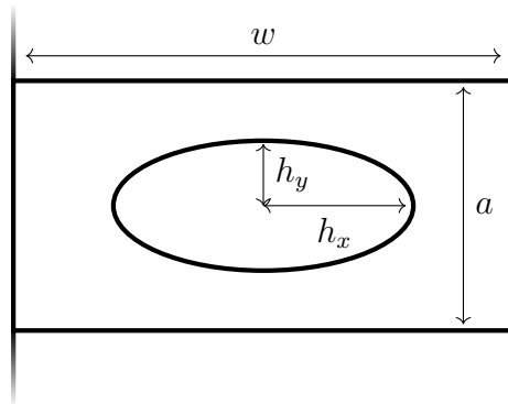
Figure 2.1: Top down view of unit cell of a phononic crystal. The periodicity of the waveguide is a , the width is w and h_x and h_y are the major and minor radii of the elliptic hole.
