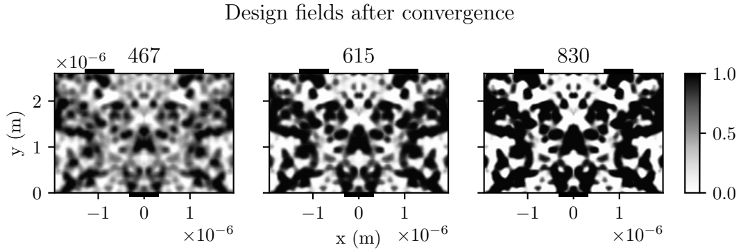
Figure 5.7: This figure shows the interpolation field at iteration 467, 615, and 830. It is clearly seen that the device becomes closer and closer to being binary.
