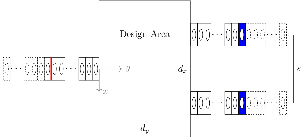
Figure 4.1: Device design to be optimized. At the red line, a wave traveling right was excited. The output was measured over the blue unit cells. The dashed unit cells marks Perfectly Matched Layers (PMLs). The large, rectangular design area has dimensions d_x \times d_y \times h .
