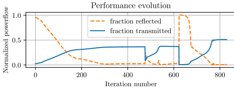
Figure 5.6: Similar to figure 5.4, but at iteration 467 and 615, a sigmoid function was abruptly applied to the design field, which causes the performance to dip as the design is perturbed. The final device was a near perfect beamsplitter, with less than 1 % of the power begin reflected, and nothing being scattered into other modes.
