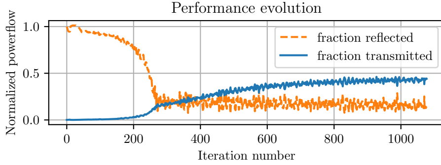
Figure 5.8: Performance evolution of the level-set device during optimization. The curve is not as smooth as the curve from the continuous optimization, which indicates that the step size is closer to being too large.
