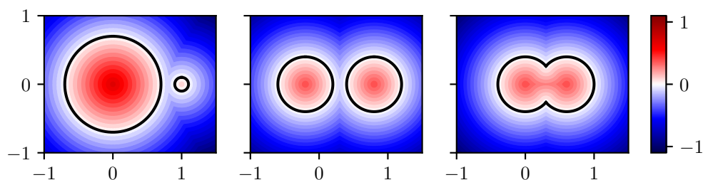
Figure 4.5: Signed distance function for the boundaries in figure 4.4. The resolution of the boundary depends only on the resolution of the signed distance field, and not on how the boundary moves, so evolving boundaries will never become poorly resolved. Additionally, topological changes are also smoothly handled since there is no need to explicitly specify connectivities.
