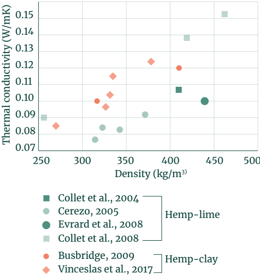
Fig.51 Thermal conductivity measurements based on density.
