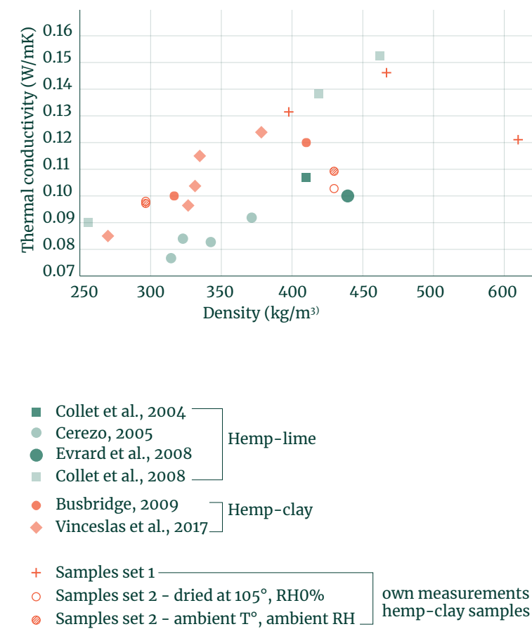
Fig.61 Thermal conductivity values of different hemp-lime and hemp-clay values from research, compared to own measurements.
