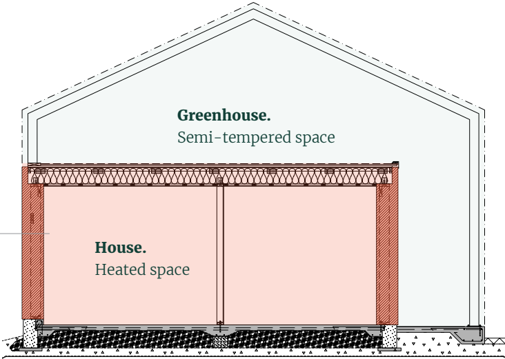
Fig.13 Transversal section –Courtesy of © Patrik Bengtsson
