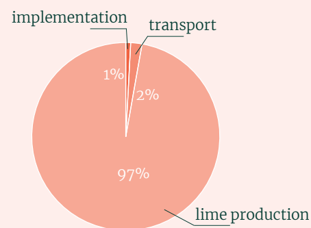
Fig.45 CO 2 emisisions hempcrete*
