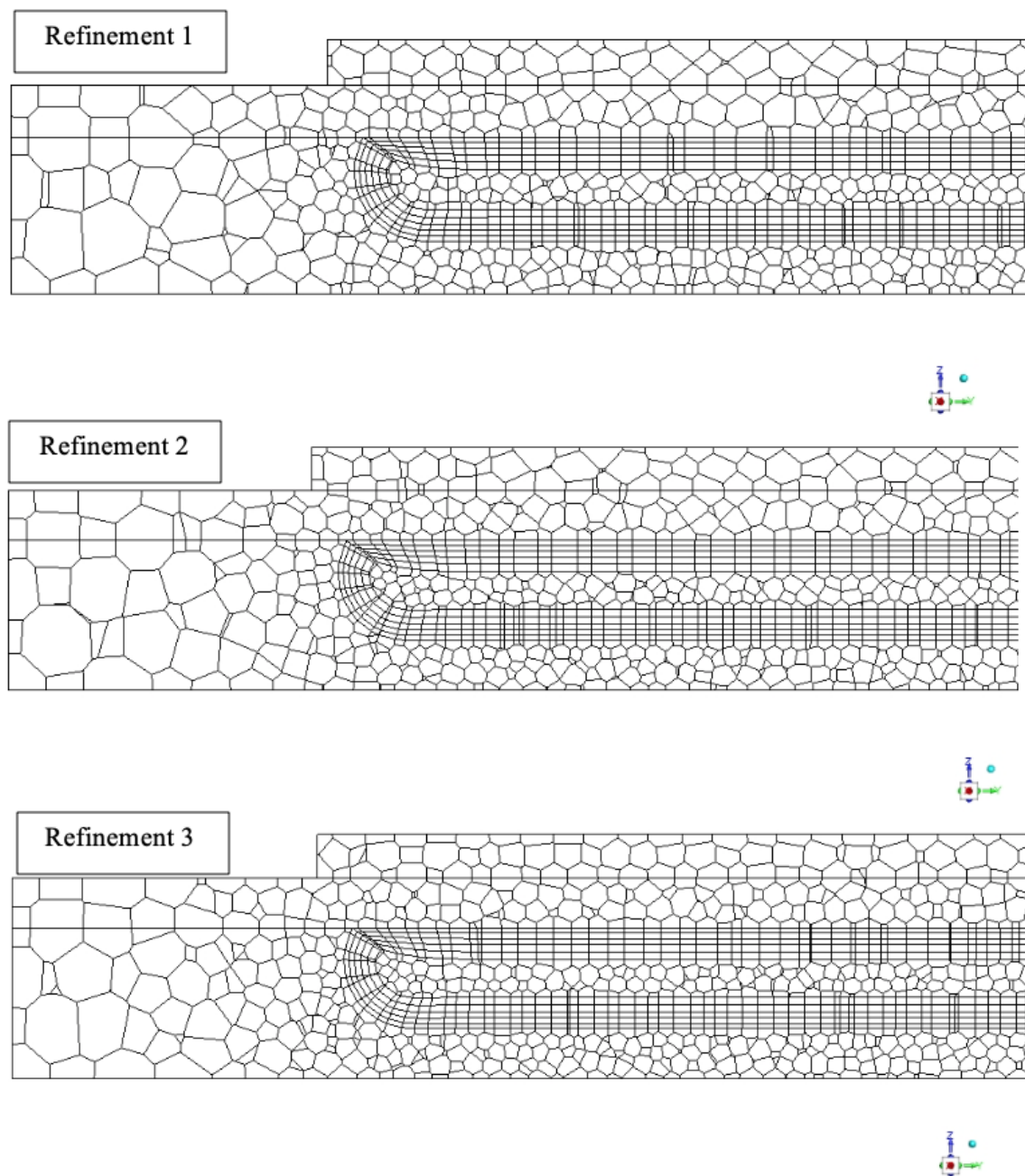
Figure B.5: A figure showing the three steps of refinement of the fin case. Taken in a cross section just after the U-turn which was assigned an area of interest.
