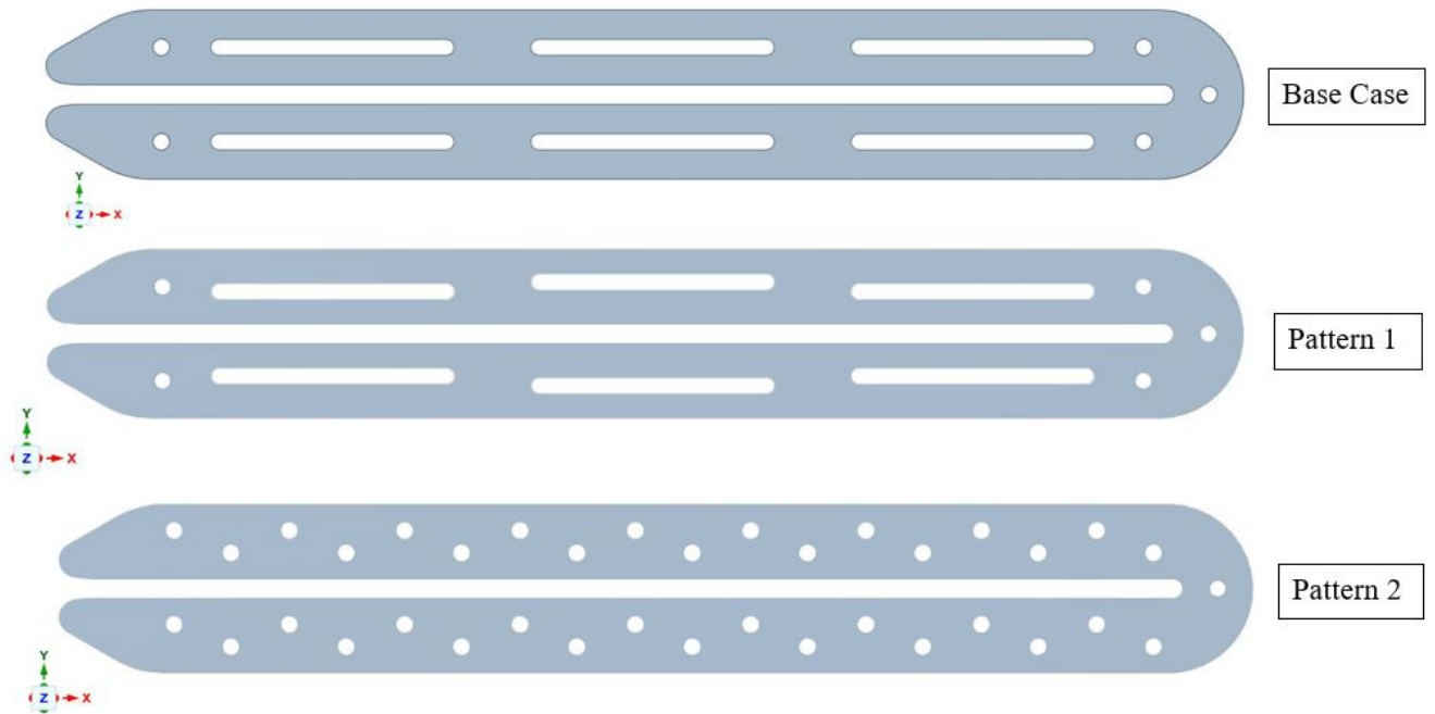
Figure 3.5: Comparison between the flow channels of the base case with the first new pattern where the same structures was used. In pattern 1 the flow channels were moved slightly so the structures were not places in a perfect row. The final second new pattern 2 was inspired by tube banks.
