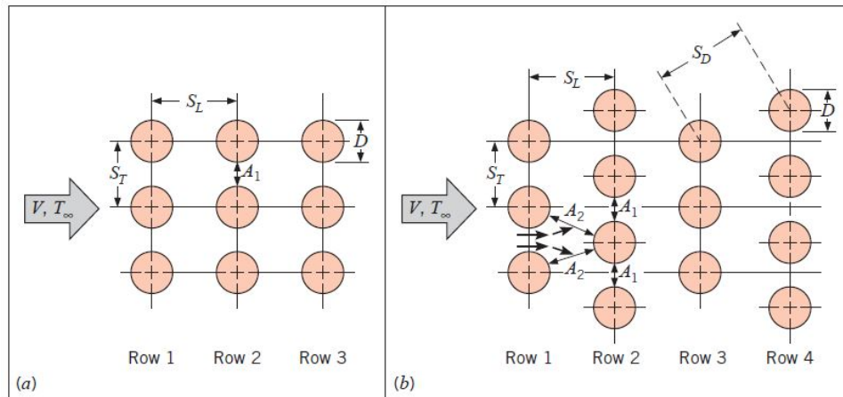
Figure 3.6: Tube arrangement in heat exchangers with tube banks. (a) Aligned. (b) Staggered [34]
