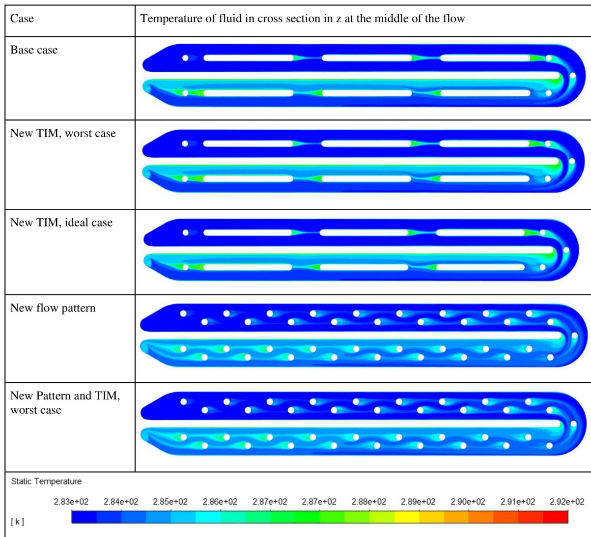
Figure 4.7: Comparative contours for all cases except the one with a fin, over the temperature distribution in the fluid, taken at a the z plane in the middle of the flow channels. With a common scale to enable comparison.
