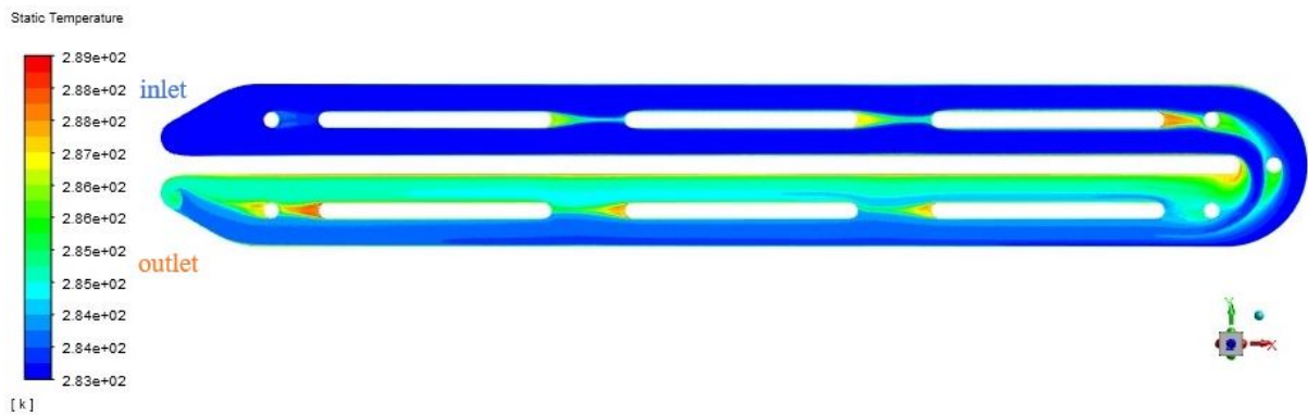
Figure D.1: A contour of the temperature of the fluid in a plan in the middle of the flow in z-direction for the base case. Side of inlet respectively outlet is marked.
