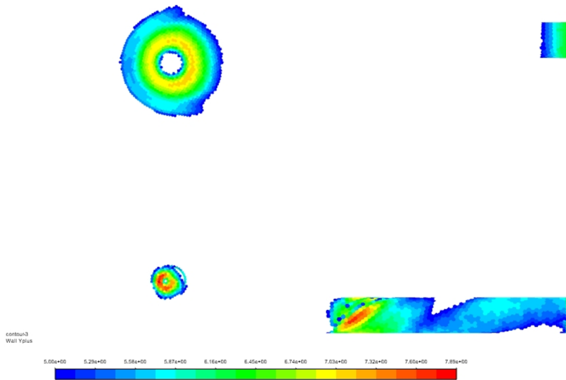
Figure A.3: y^+ above five which is outside the given limit. To the right from the side, and to the left from above
