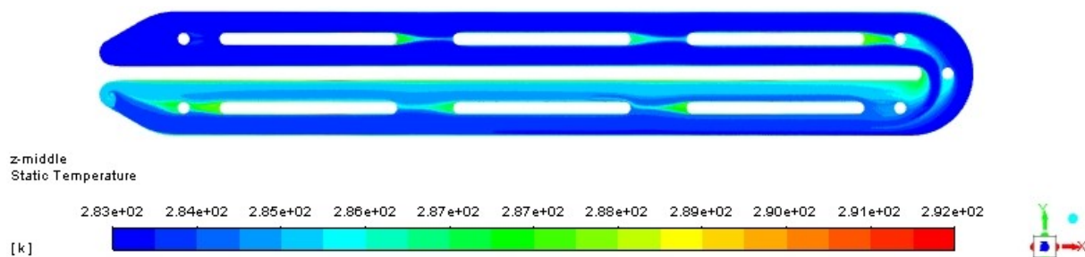
Figure 4.10: Contours of the fin case showing the temperature distribution in the fluid in z-direction.
