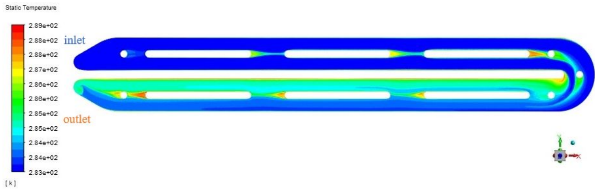
Figure 4.3: A contour of the temperature of the fluid in z-direction, in the plane at the middle of the flow. Side of inlet respectively outlet is marked.
