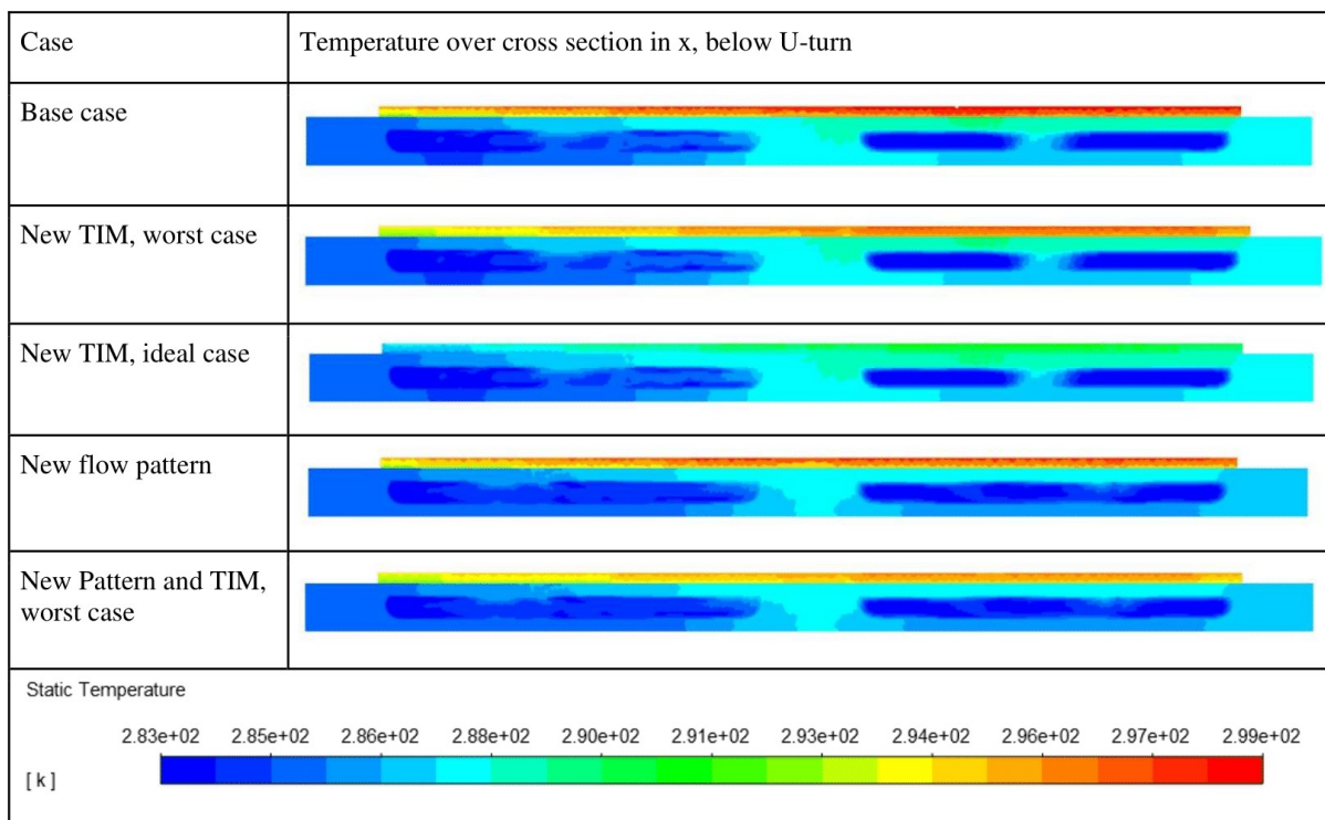
Figure 4.5: Comparative contours for all cases except the fin case, over the temperature distribution taken at a plane in x-direction below the U-turn. With a common scale to enable comparison.
