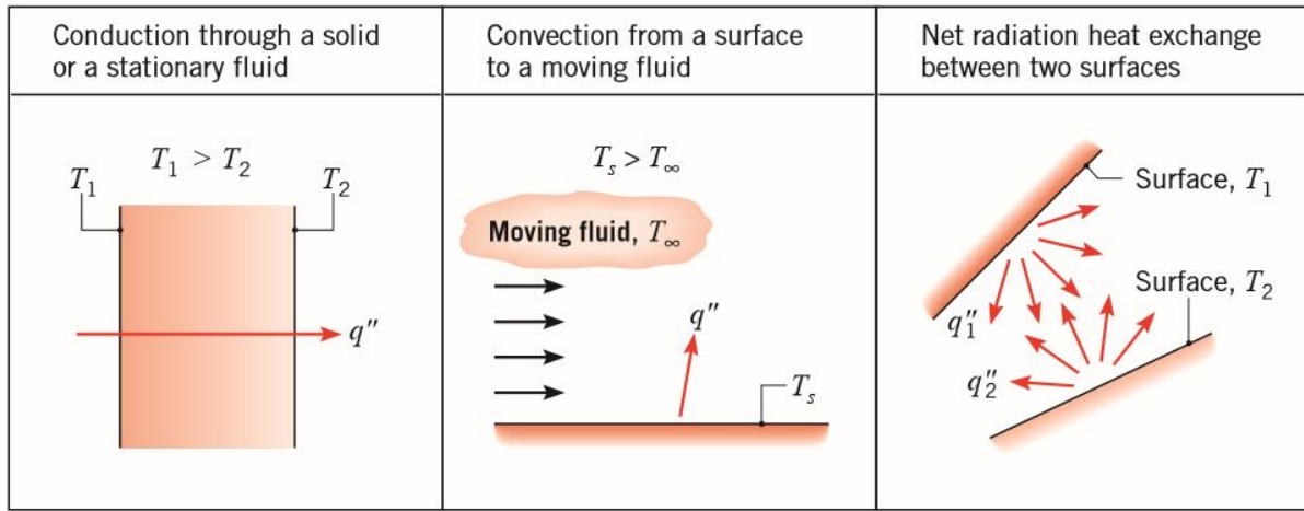
Figure 2.1: A simple illustration of the three heat transfer modes conduction, convection, and radiation. Short descriptions of the three modes are included. The temperature difference, the driving force, and the heat flux, q'' , is marked in all three cases. [34]
