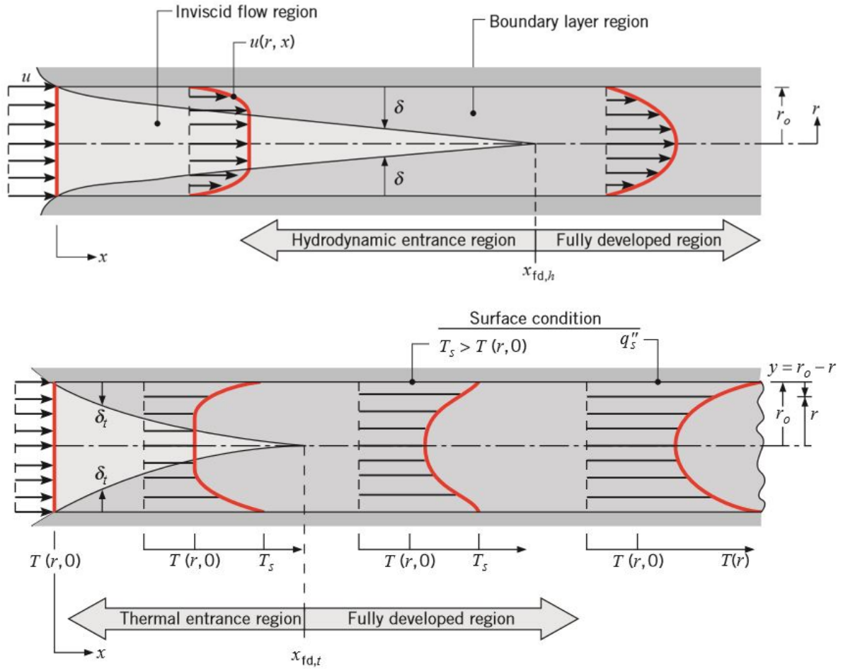
Figure 2.5: First illustration is of how a laminar velocity boundary layer develop in a circular tube. Below is the corresponding development of a thermal boundary in a similar heated circular tube.[34]
