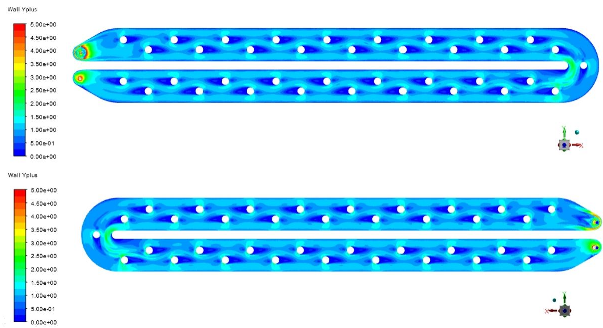
Figure C.2: Wall y^+ from above and from below for the new case with different pattern, with a scale from zero to five
