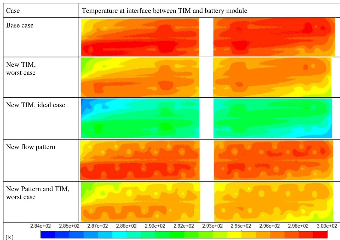
Figure 4.6: Comparative contours for all cases, except the one with a fin, over the temperature distribution over the interface between the TIM and the battery module. With a common scale to enable comparison.
