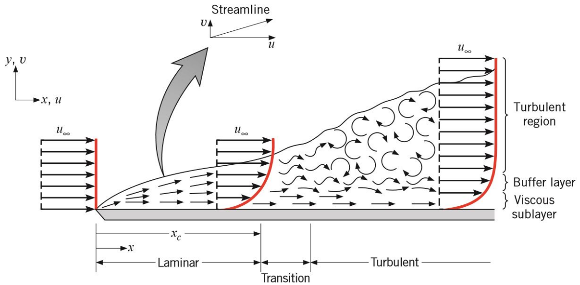
Figure 2.3: Development of velocity boundary layer on a flat plate. Including the three regions viscous sublayer, buffer layer and turbulent region of a fully developed flow. [34]
