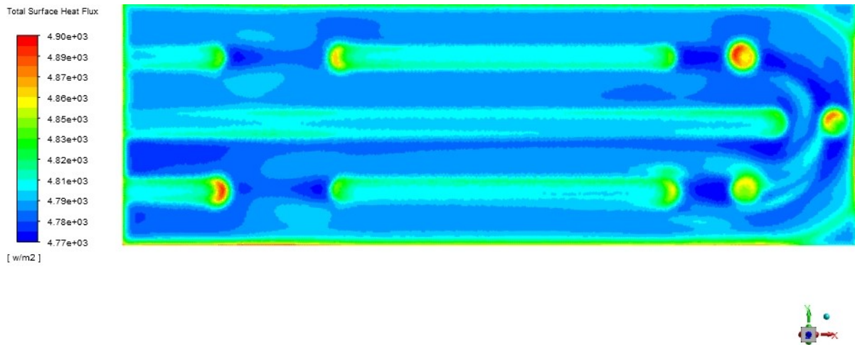
Figure 4.4: A contour of the total surface heat flux at the interface between one of the thermal pads and the cooling plate.
