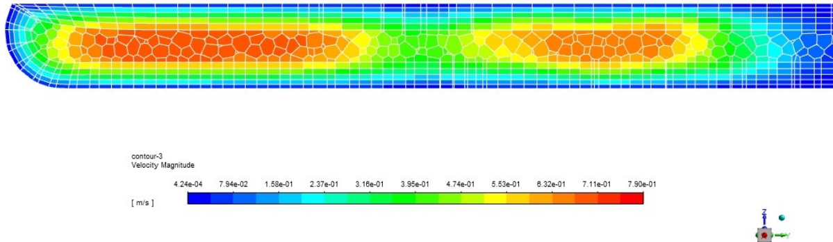
Figure C.1: Contour of the velocity field in a cross section in x direction including the mesh. Confirms that the total height of the mesh boundary layer capture the velocity field height of the boundary layer for the new pattern.
