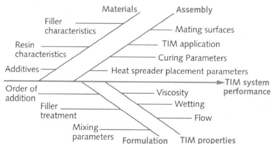
Figure 2.7: A fish-bone diagram over important material properties influencing the performance of a thermal interface material (TIM), to illustrate the complexity of choosing and evaluating a TIM. [53]
