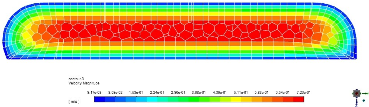
Figure A.1: Contour of the velocity field in a cross section in x direction including the mesh. Confirms that the total height of the mesh boundary layer capture the velocity field height of the boundary layer.
