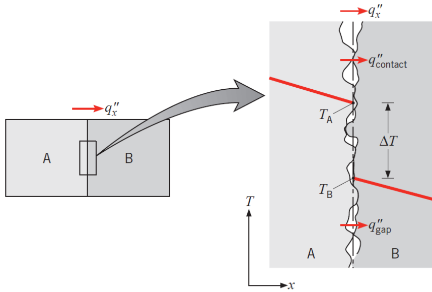
Figure 2.2: A zoom in to illustrate how surface roughness lead to imperfect contact and therefore air voids between two surfaces. The air have an isolating effect which lead to a temperature drop over the interface. So, the heat flux where there is contact, q_{\text{contact}}'' , is larger than where there are a gap, q_{\text{gap}}'' and an average heat flux q_x'' is reached. [34].
