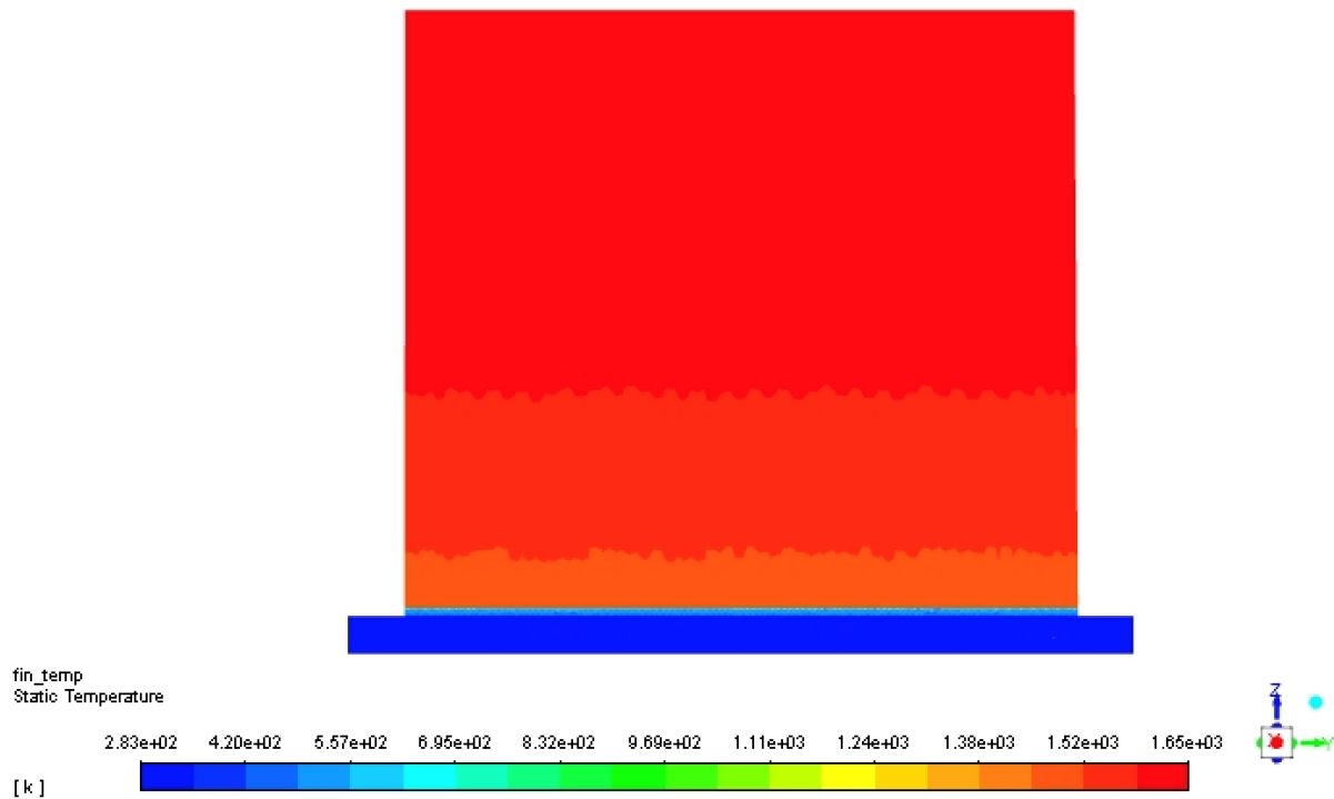
Figure 4.9: Contours of the fin case showing the temperature distribution over the fin in x-direction.
