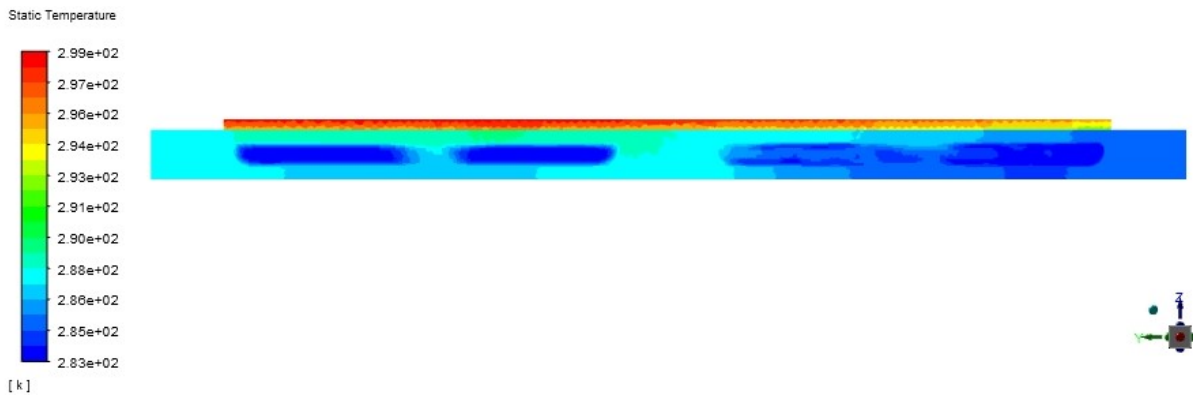
Figure 4.1: A contour of the temperature distribution through a cross section just below the U-turn. It can be seen that the highest temperature of the thermal pad surface occur where the heat flux was applied.
