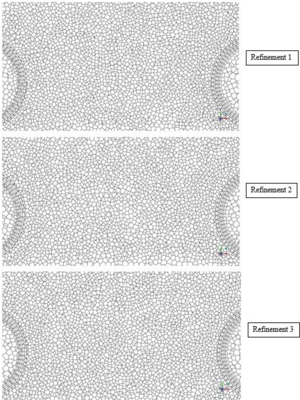
Figure A.4: Three steps of refinement of the Base Case. The picture is taken in the middle of the flow in z-led and just after the U-turn which was assigned an area of interest.
