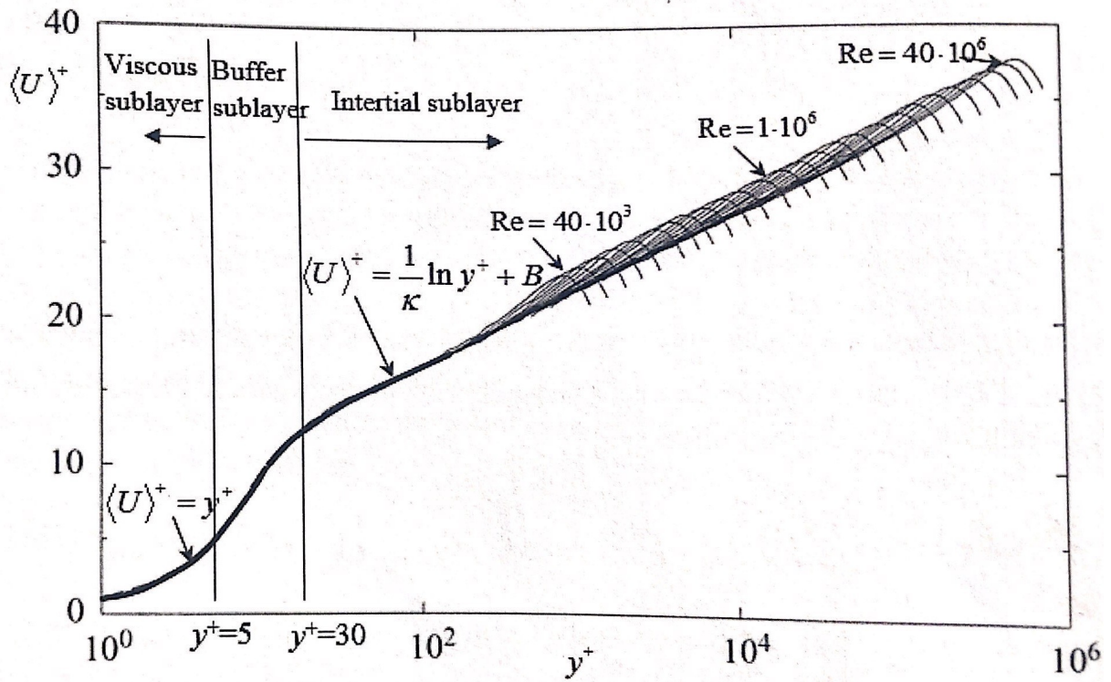
Figure 2.4: Graph of the boundary layer marking the viscous sublayer, buffer sublayer and the inertial sublayer with respective limiting value for y^+ [51]
