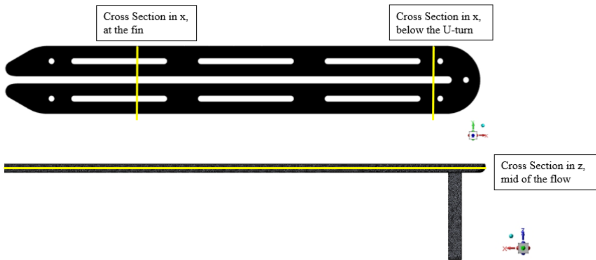
Figure 3.7: Cross sections in the two of the three directional dimensions which were used to present the result of the analysis of the cases. First is two planes in x and then one in z.
