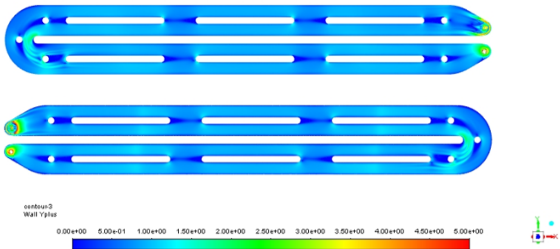
Figure B.2: Wall y^+ from above and from below for the fin case, with a scale from zero to five
