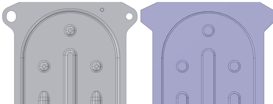
Figure 3.3: Example of how the cooling plate constructing the flow channels were simplified by removing small features. To the left is the original and to the right is the simplified geometry
