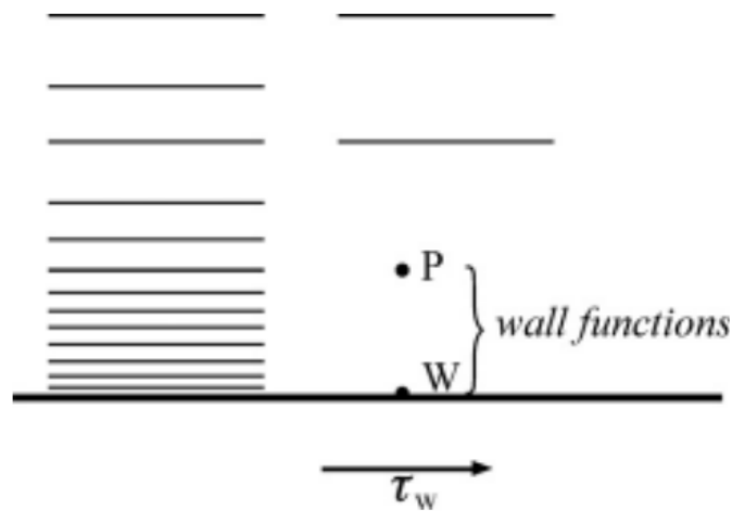
Figure 2.6: How wall functions is applied at a distance from the wall, where point P correspond to the position of W outside of the boundary layer [51]
