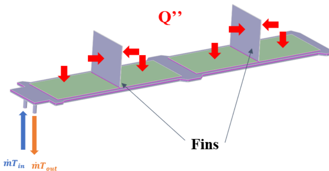
Figure 3.4: Layout of how the fins were placed in the model used in the simulations. Marking heat flux, Q'' , mass flow, \dot{m} , inlet temperature, T_{in} and outlet temperature, T_{out} .
