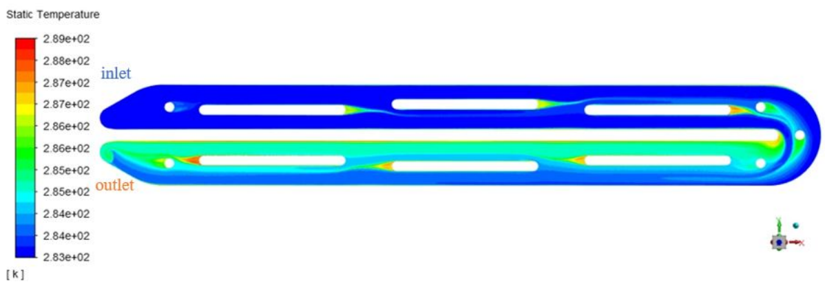
Figure D.2: A contour of the temperature of the fluid in a plan in the middle of the flow in z-direction for pattern 1. Side of inlet respectively outlet is marked.
