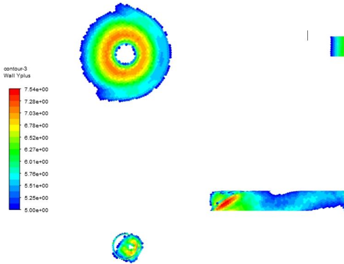
Figure C.3: y^+ above five which is outside the given limit. To the right from the side, and to the left from above
