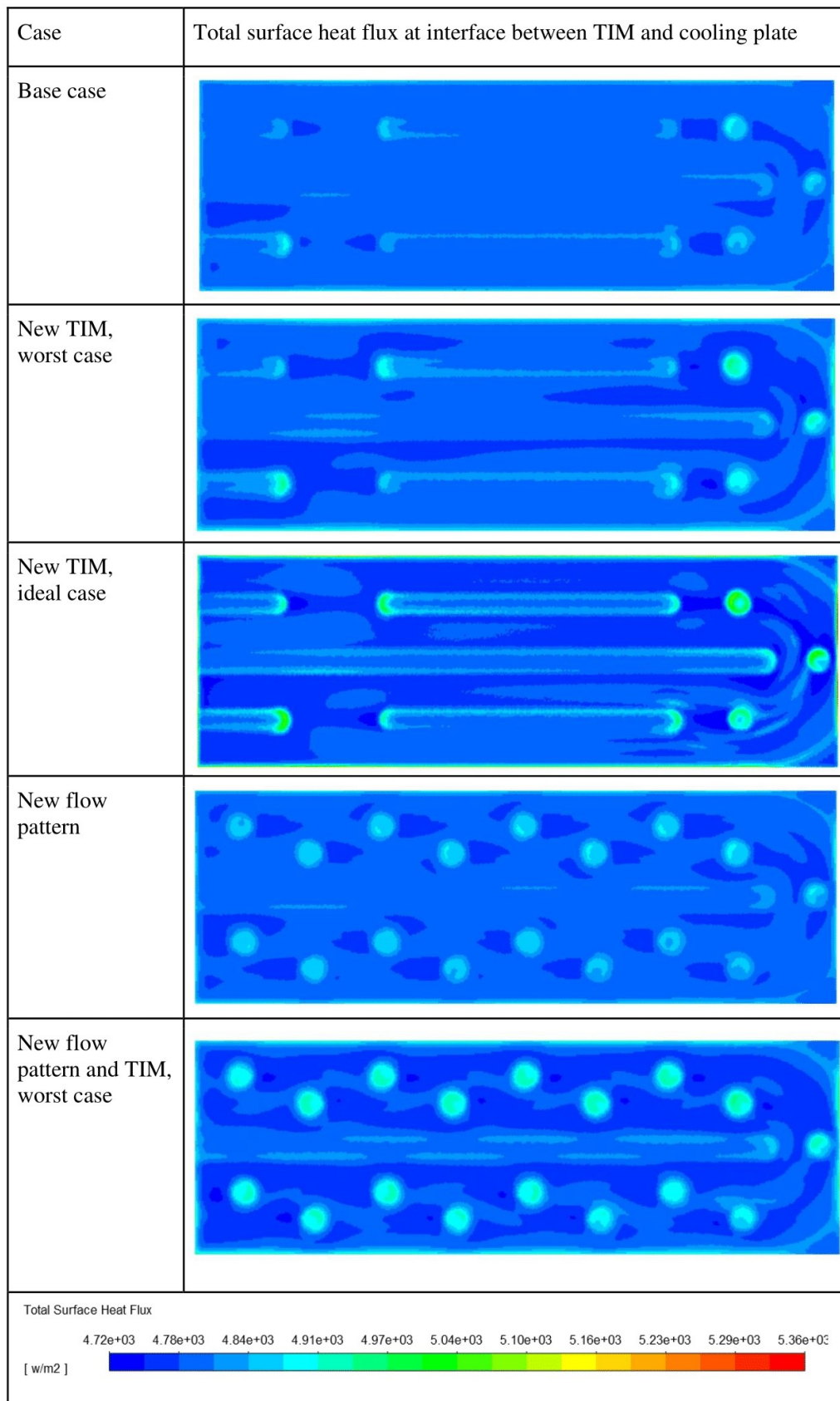
Figure 4.8: Comparative contours for all cases, except the one with a fin, over the heat transfer rate at the interface between the TIM and the cooling plate. With a common scale to enable comparison.
