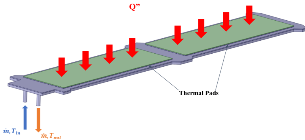
Figure 3.2: Overview of the simplified model for two out of eight battery modules removed from on top of the pads. Marking heat flux, Q'' , mass flow, \dot{m} , inlet temperatures, T_{in} , outlet temperature, T_{out} and location of pads.
