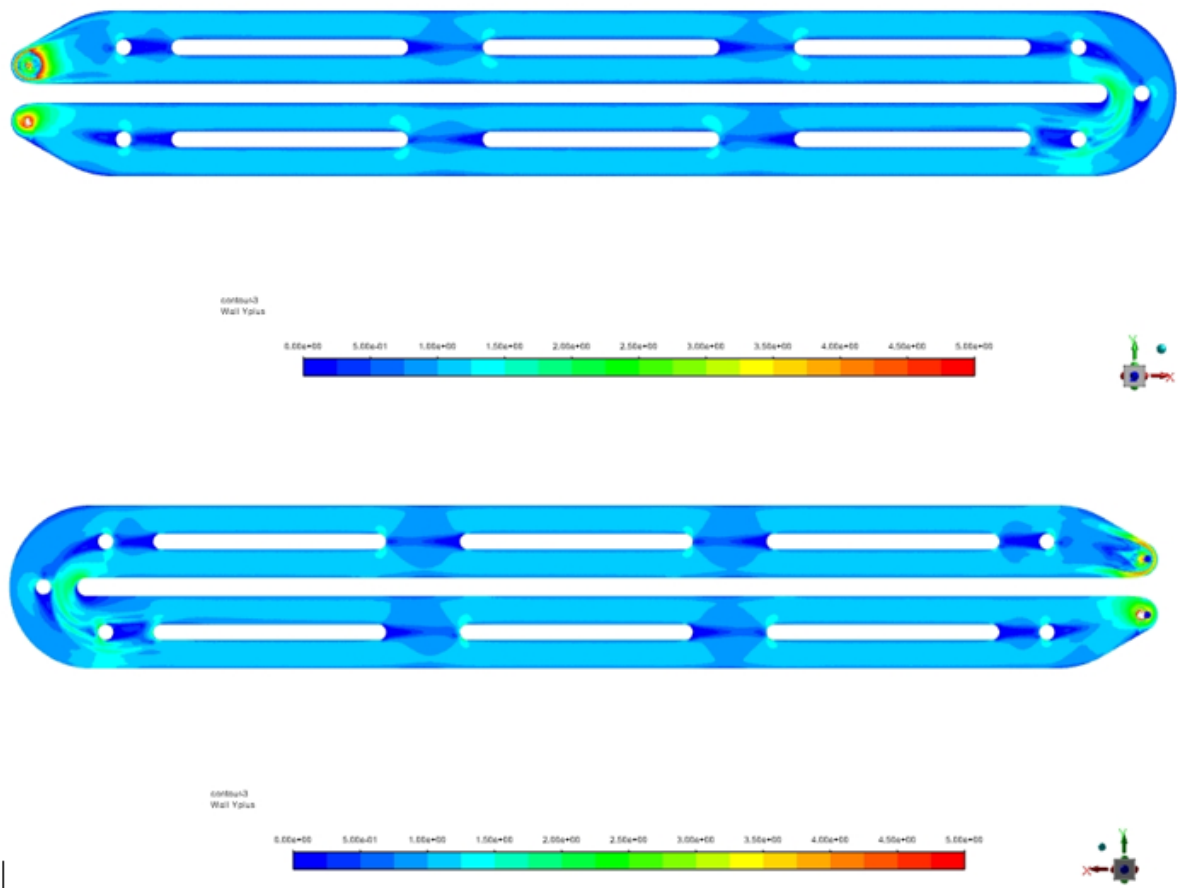
Figure A.2: Wall y^+ from above and from below for the Base Case, with a scale from zero to five
