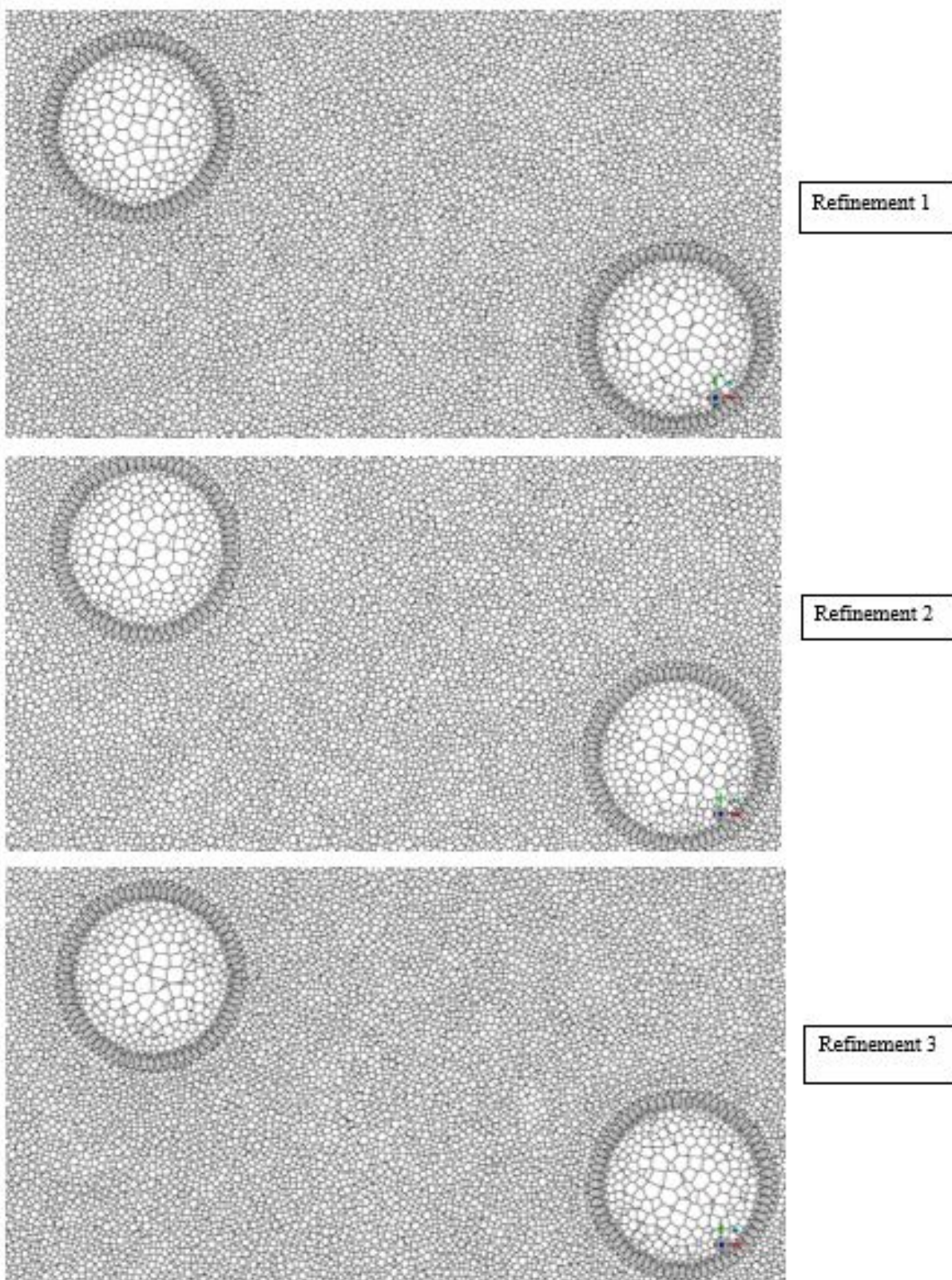
Figure C.4: Three steps of refinement of the New case with a different pattern. The picture is taken in the middle of the flow in z-led and just after the U-turn which was assigned an area of interest.
