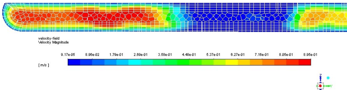
Figure B.1: Contour of the velocity field in a cross section in x direction including the mesh. Confirms that the total height of the mesh boundary layer capture the velocity field height of the boundary layer for the fin case.
