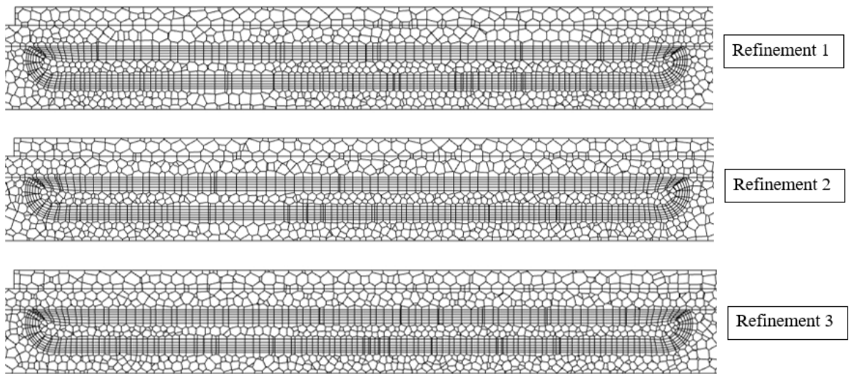
Figure A.5: Three steps of refinement of the Base Case. Picture taken in a cross section just after the U-turn which was assigned an area of interest.
