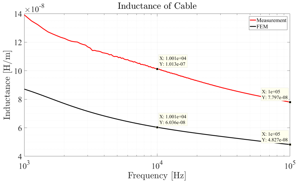
Figure 4.6: Comparison of inductance for 50 \text{ mm}^2 cable
