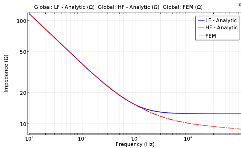
Figure 4.4: Analytical and simulated result for impedance of 50 mm 2 cable
