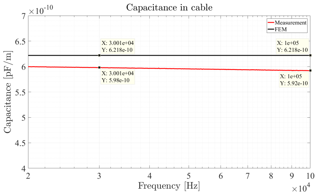
Figure 4.7: Comparison of capacitance for 50 \text{ mm}^2 cable
