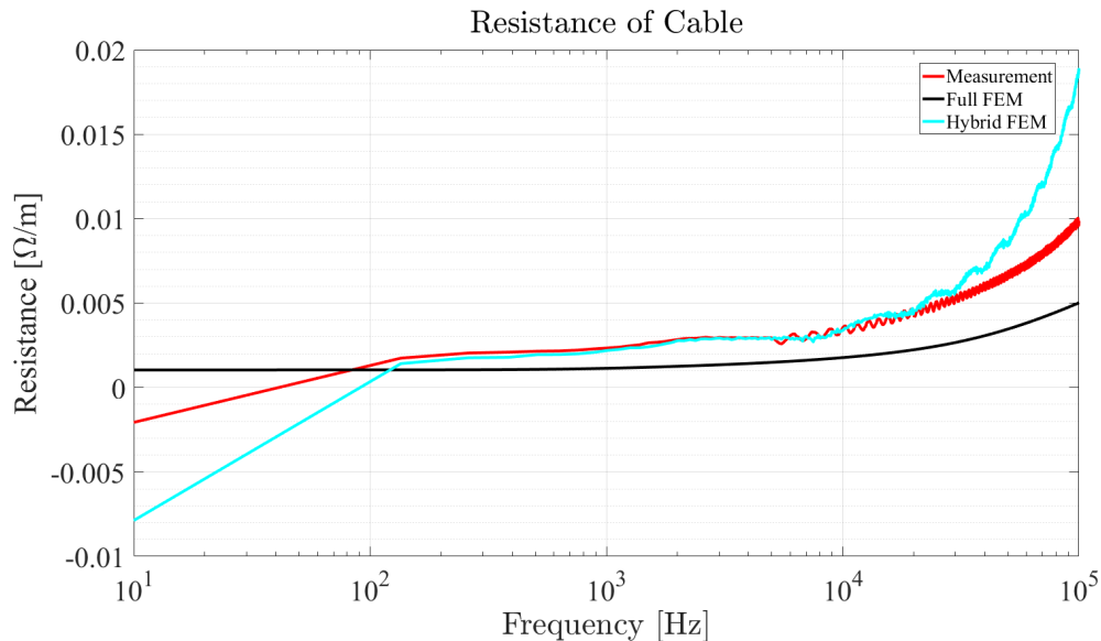
Figure 4.5: Comparison of resistance for 50 \text{ mm}^2 cable
