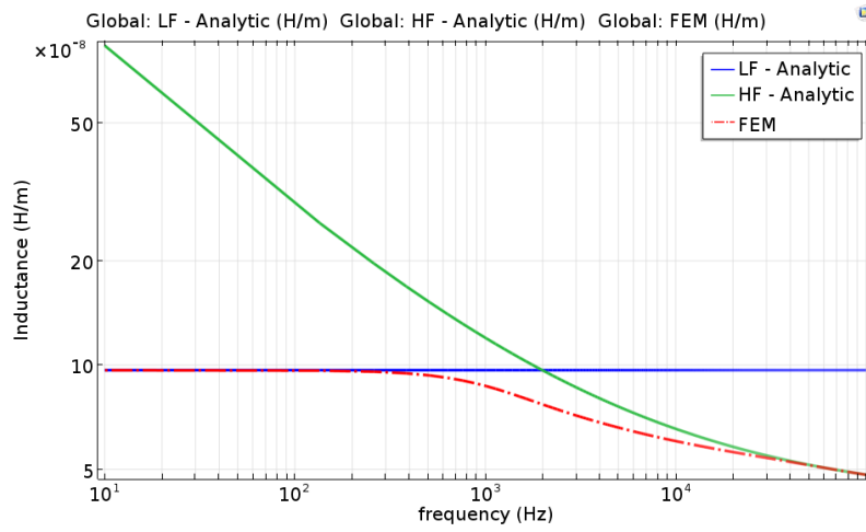
Figure 4.2: Analytical and simulated result for inductance of 50 mm 2 cable
