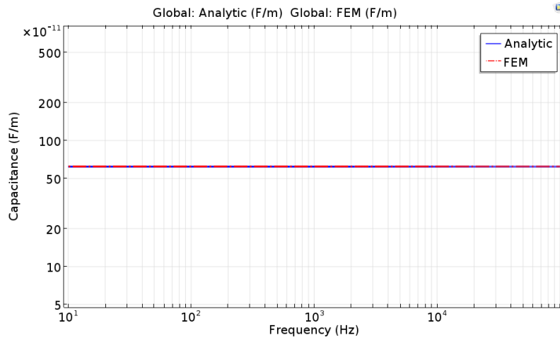
Figure 4.3: Analytical and simulated result for capacitance of 50 mm 2 cable
