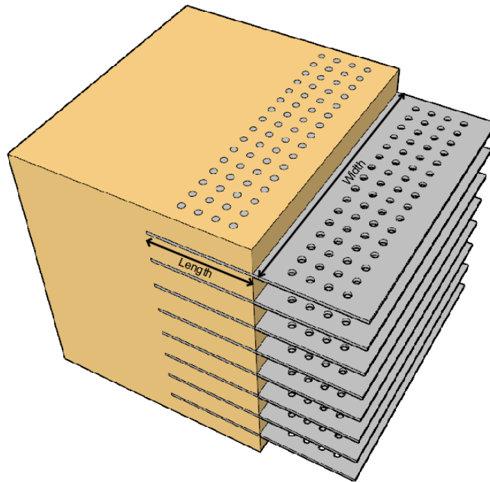
Figure 4.1: Slotted-in steel plate connection with the length and width of the plate explained.
