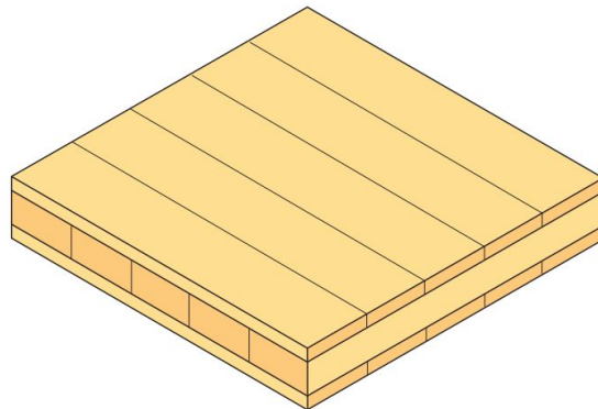
Figure 2.4: Cross-laminated timber (Swedish Wood, 2016a).
