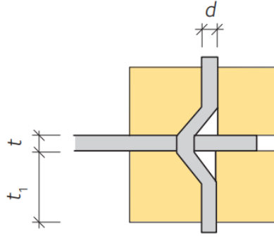
Figure 2.23: Failure mode to Equation 2.32 (Swedish Wood, 2016a).
