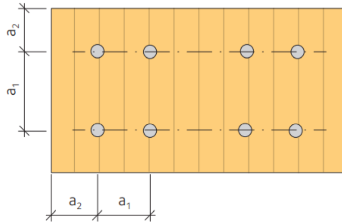
Figure 2.26: Minimum distances glued-in rods (Swedish Wood, 2016d).
