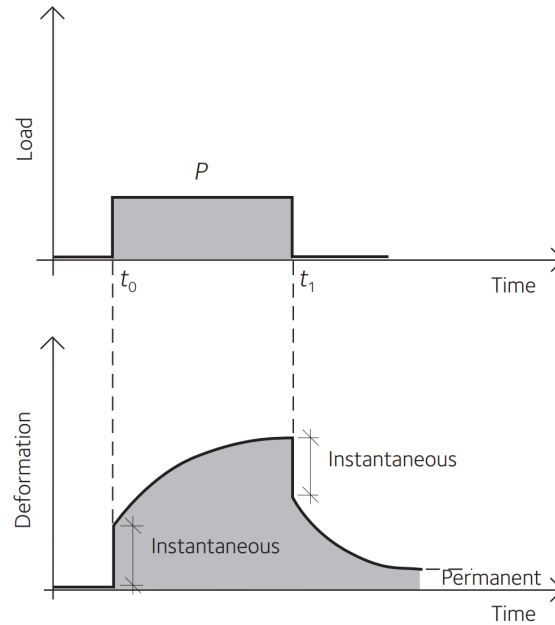
Figure 2.2: Effect of creep over time (Swedish Wood, 2016a).
