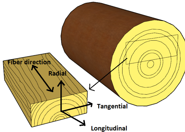
Figure 2.1: The grain directions in wood.
