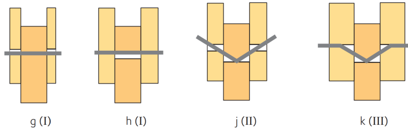
Figure 2.20: Failure modes double shear (Swedish Wood, 2016a).
