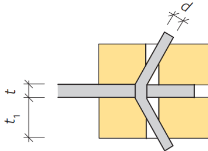
Figure 2.22: Failure mode to Equation 2.31 (Swedish Wood, 2016a).
