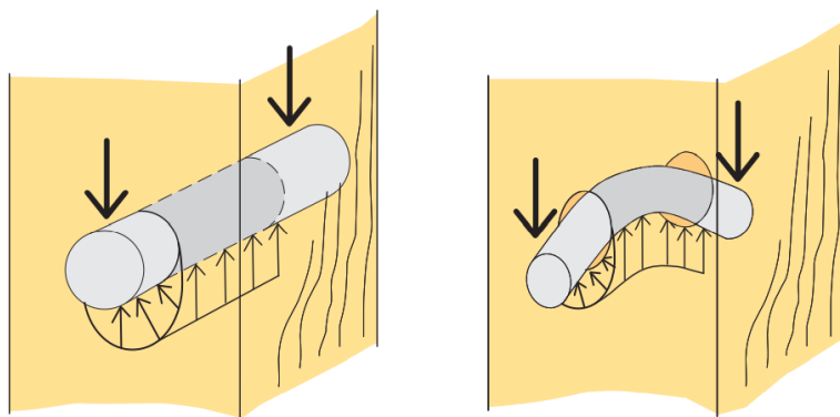
Figure 2.14: Dowel action (Swedish Wood, 2016a).
