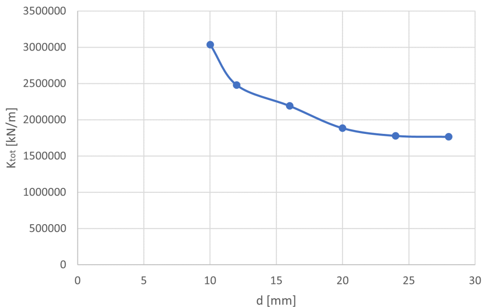
Figure 5.4: Change of stiffness with varying dowel dimensions.
