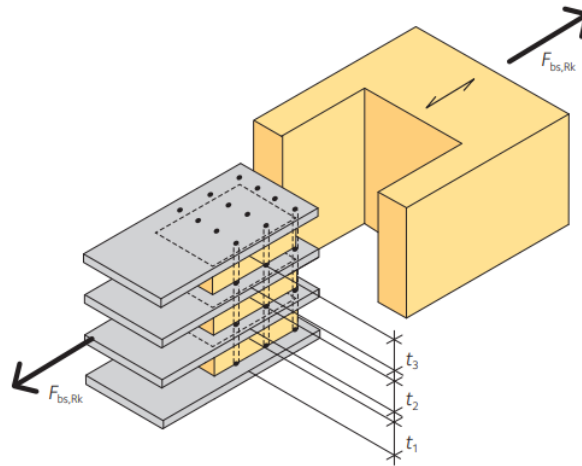
Figure 2.16: Block shear failure (Swedish Wood, 2016a).
