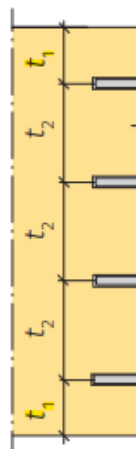
Figure 2.25: Minimum distances t_1 and t_2 (Swedish Wood, 2016d).
