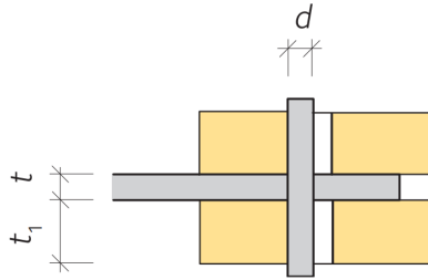
Figure 2.21: Failure mode to Equation 2.30 (Swedish Wood, 2016a).
