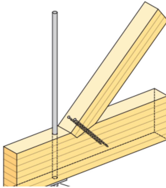
Figure 2.11: Contact joint with supplementary fasteners (Swedish Wood, 2016a).
