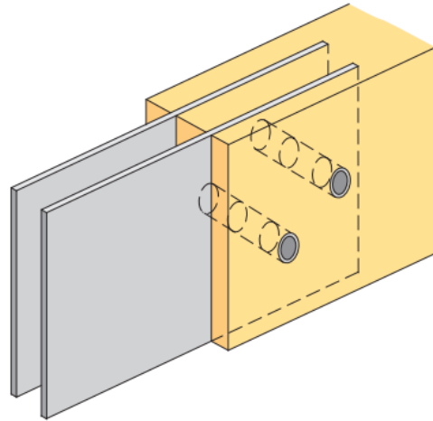
Figure 2.12: Slotted-in steel plates (Swedish Wood, 2016d).
