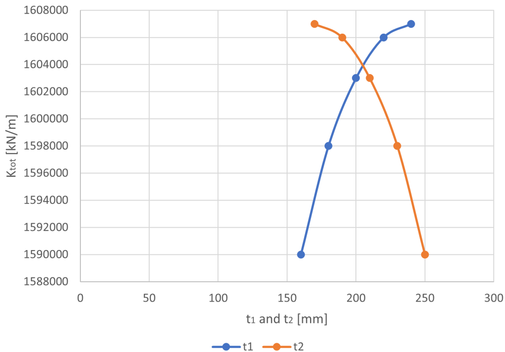
Figure 5.7: Change of stiffness with varying distance between plates.
