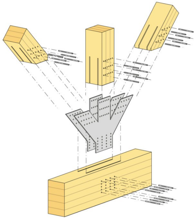
Figure 6.1: Example of a slotted-in steel joint with several connecting beams (Croce, 2016).
