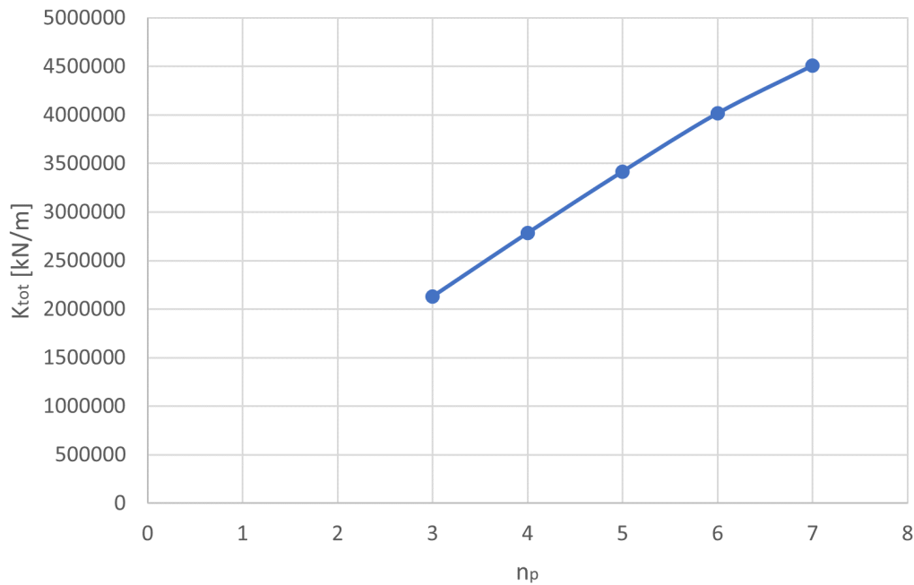
Figure 5.5: Change of stiffness with varying number of plates.
