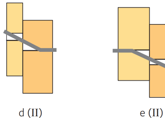
Figure 2.18: Failure mode II (Swedish Wood, 2016a).
