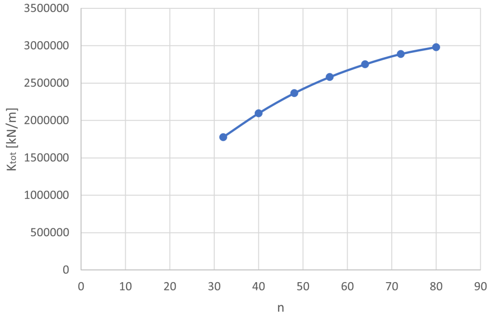
Figure 5.3: Change of stiffness with varying number of dowels.
