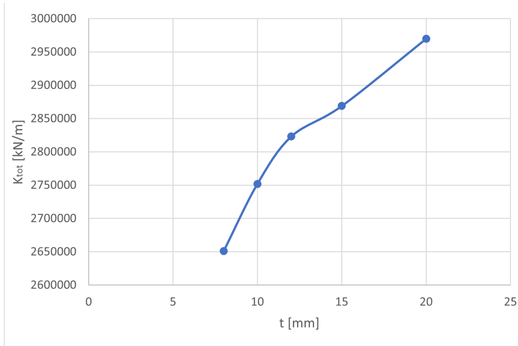
Figure 5.6: Change of stiffness with varying plate thickness.
