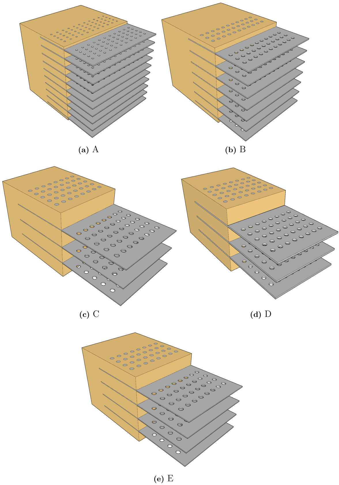
Figure 5.1: Connections A-E.
