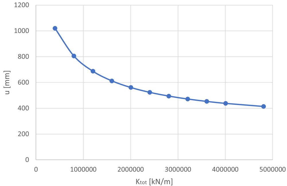
Figure 5.2: Displacement changes with varying stiffness.
