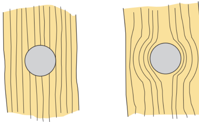
Figure 2.15: Predrilling, embedment strength (Swedish Wood, 2016a).
