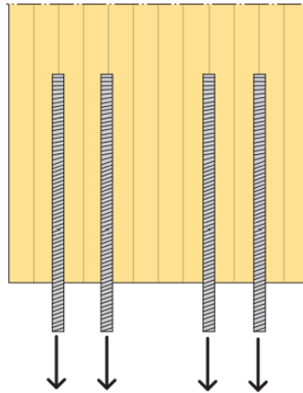
Figure 2.10: Glued-in rods (Swedish Wood, 2016d).
