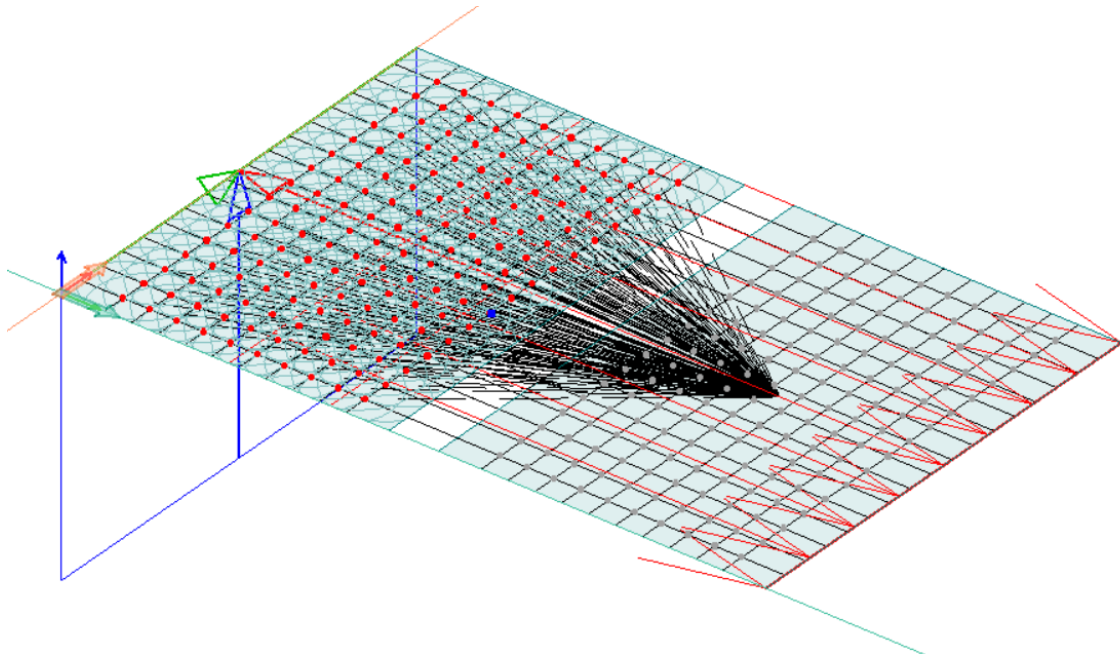
Figure 4.2: Example if a connection modelled in FEM-design.
