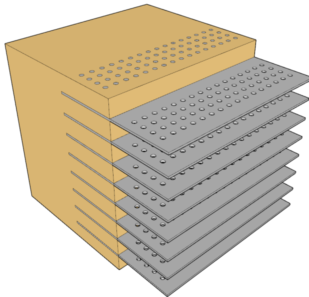
Figure 5.11: Design of the final connection.
