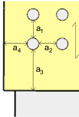
Figure 2.24: Minimum distances between fasteners a_1 , a_2 , a_3 and a_4 .
