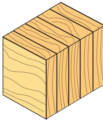
Figure 2.5: Part of a laminated veneer lumber board (Swedish Wood, 2016a).
