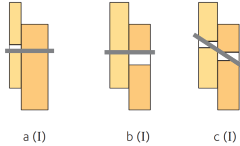
Figure 2.17: Failure mode I (Swedish Wood, 2016a).
