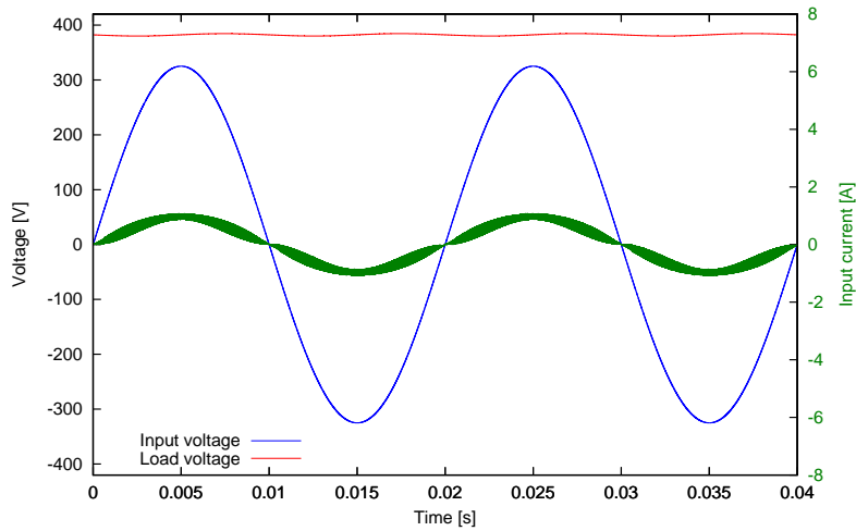
Figure 12: Voltages and currents with active PFC, with EMI filter.
