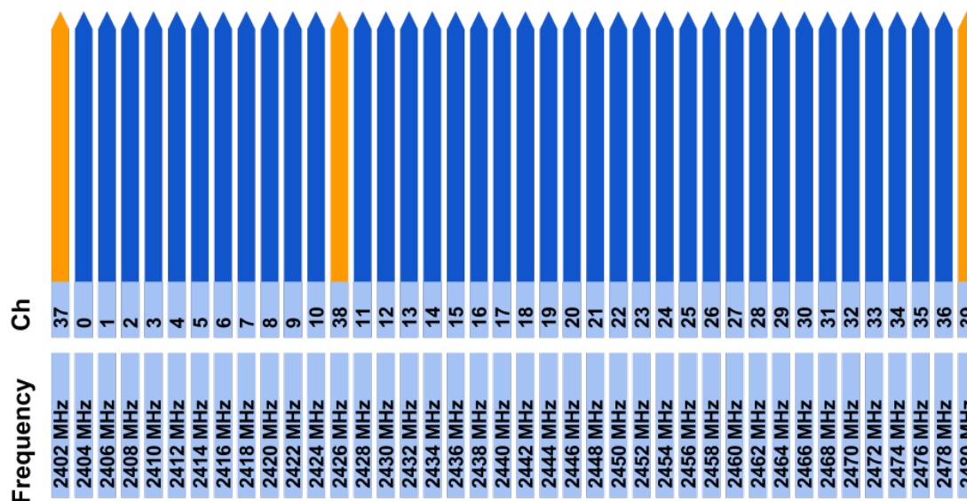
Figure 2.2: Overview of Bluetooth smart channel spectrum
