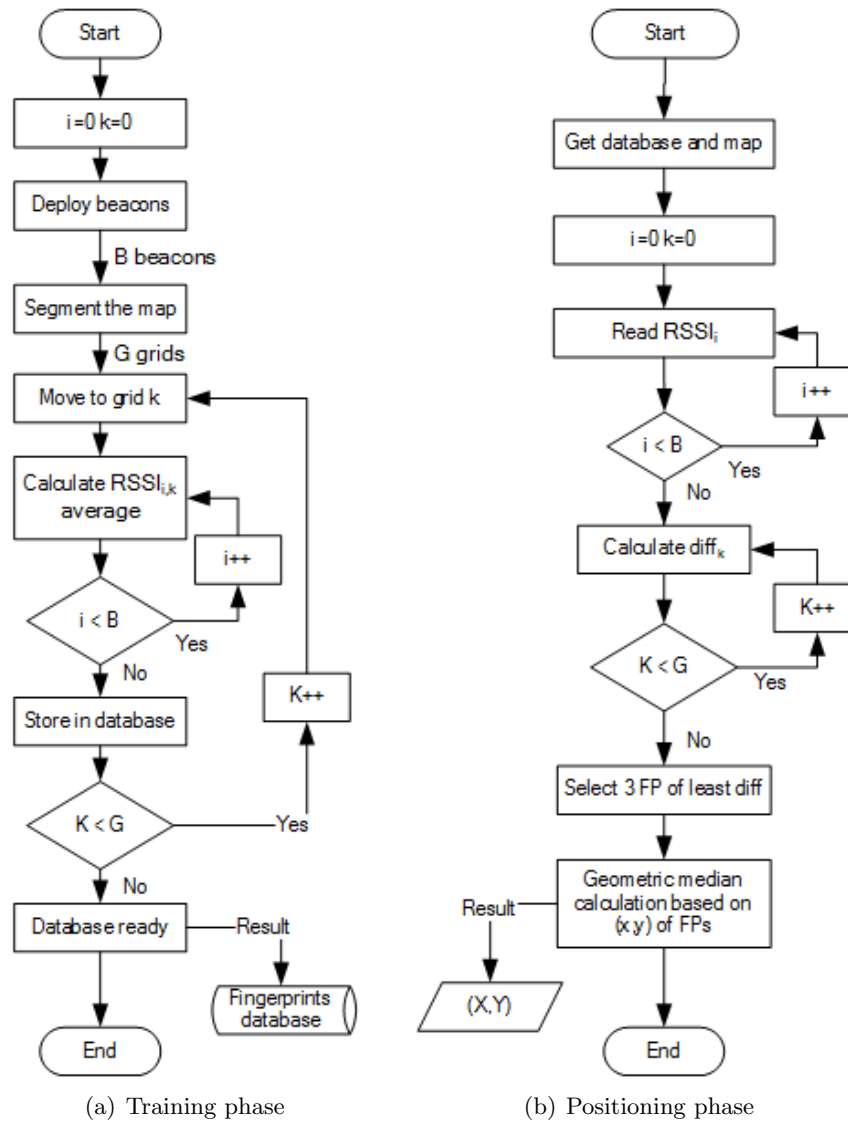
Figure 5.7: Fingerprinting flowchart
