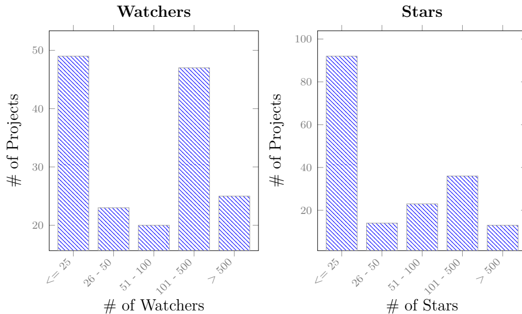
Figure 5.3: The popularity of the 166 OS Java projects as measured by the number of stars on GitHub and the number of subscribers, known as watchers.
