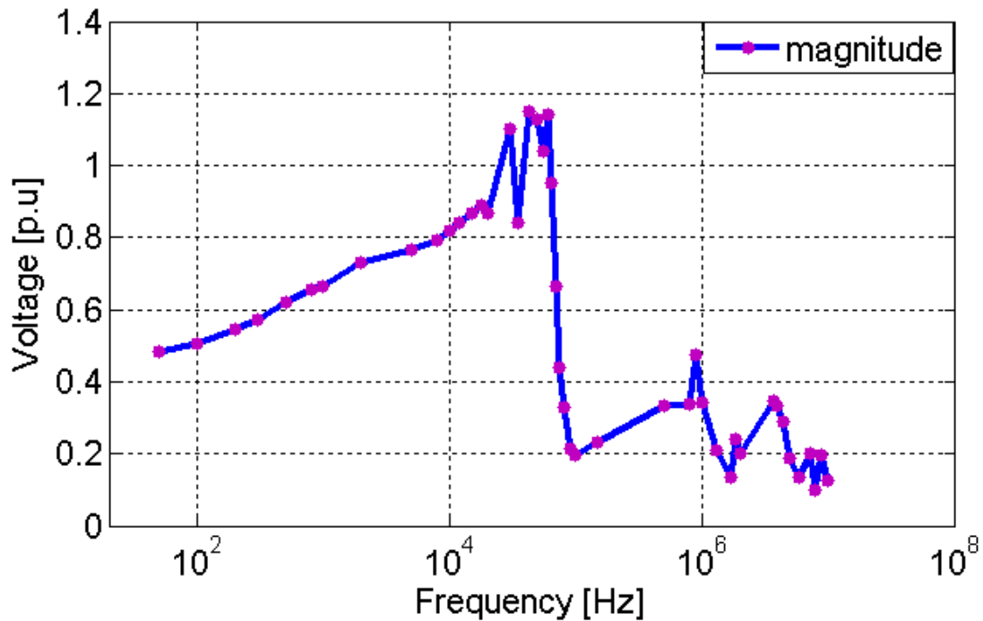
Figure 33 Voltage stress at node 1200
