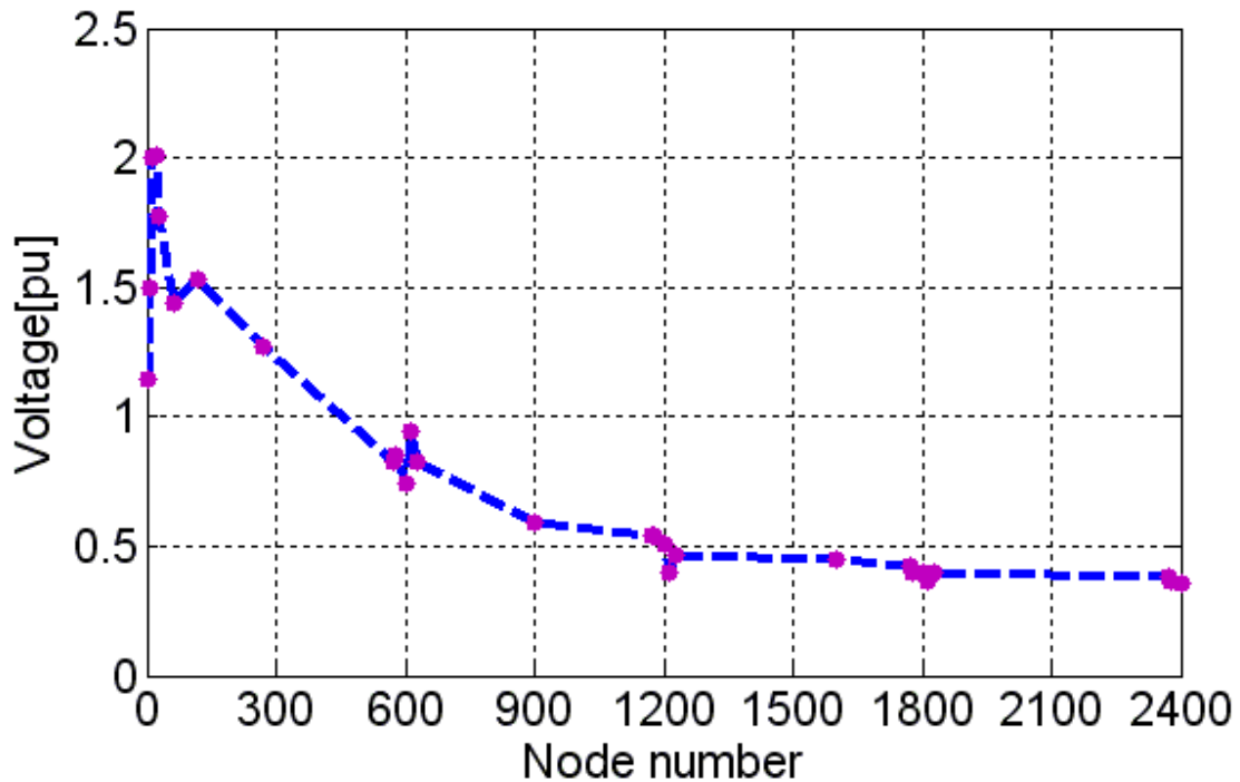
Figure 29 Voltage distribution at 5.2 MHz
