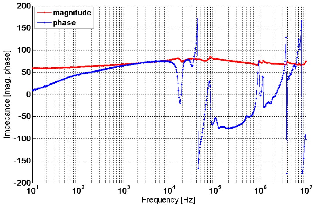
Figure 9 Impedance measurement
