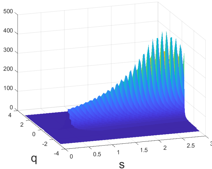
Figure 5.2: (|[Y, Y](t) - t|^2 + \mu_1 \sum_{i=1}^5 g_i(\sigma_0, s, q))^{-1} , high resolution. Note the fluctuations.
